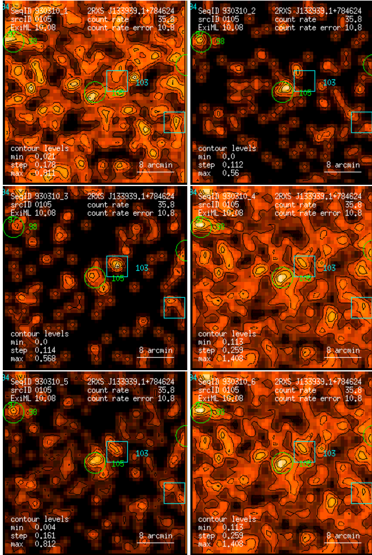
Figure 105: RASS 930310: detection 0105: band rate images, Gaussian filter: (1) PSPC channels 11 – 41, (2) 52 – 90, (3) 91 – 201, (4) 11 – 235, (5) 52 – 201, (6) 11 – 201. Broad band rates in counts/ks. Band rate contour levels in counts/ks/arcmin 2 .
