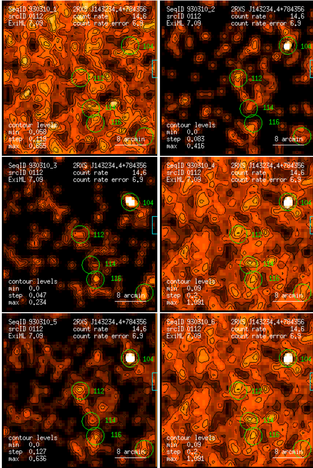
Figure 112: RASS 930310: detection 0112: band rate images, Gaussian filter: (1) PSPC channels 11 – 41, (2) 52 – 90, (3) 91 – 201, (4) 11 – 235, (5) 52 – 201, (6) 11 – 201. Broad band rates in counts/ks. Band rate contour levels in counts/ks/arcmin 2 .
