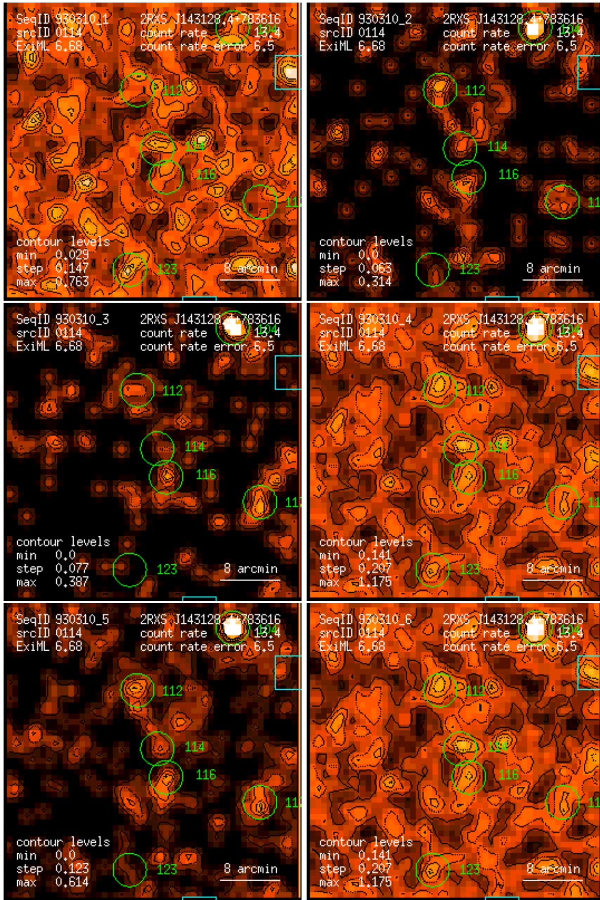
Figure 114: RASS 930310: detection 0114: band rate images, Gaussian filter: (1) PSPC channels 11 – 41, (2) 52 – 90, (3) 91 – 201, (4) 11 – 235, (5) 52 – 201, (6) 11 – 201. Broad band rates in counts/ks. Band rate contour levels in counts/ks/arcmin 2 .
