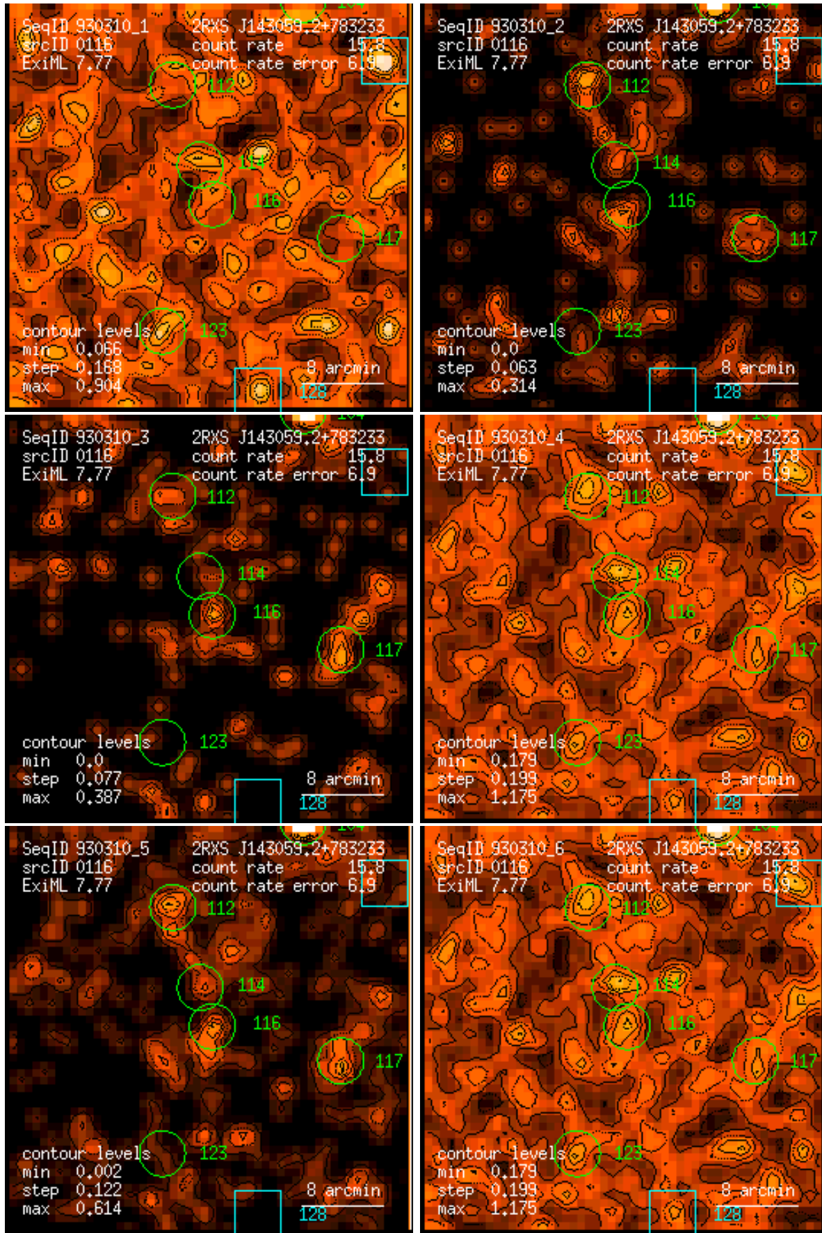
Figure 116: RASS 930310: detection 0116: band rate images, Gaussian filter: (1) PSPC channels 11 – 41, (2) 52 – 90, (3) 91 – 201, (4) 11 – 235, (5) 52 – 201, (6) 11 – 201. Broad band rates in counts/ks. Band rate contour levels in counts/ks/arcmin 2 .
