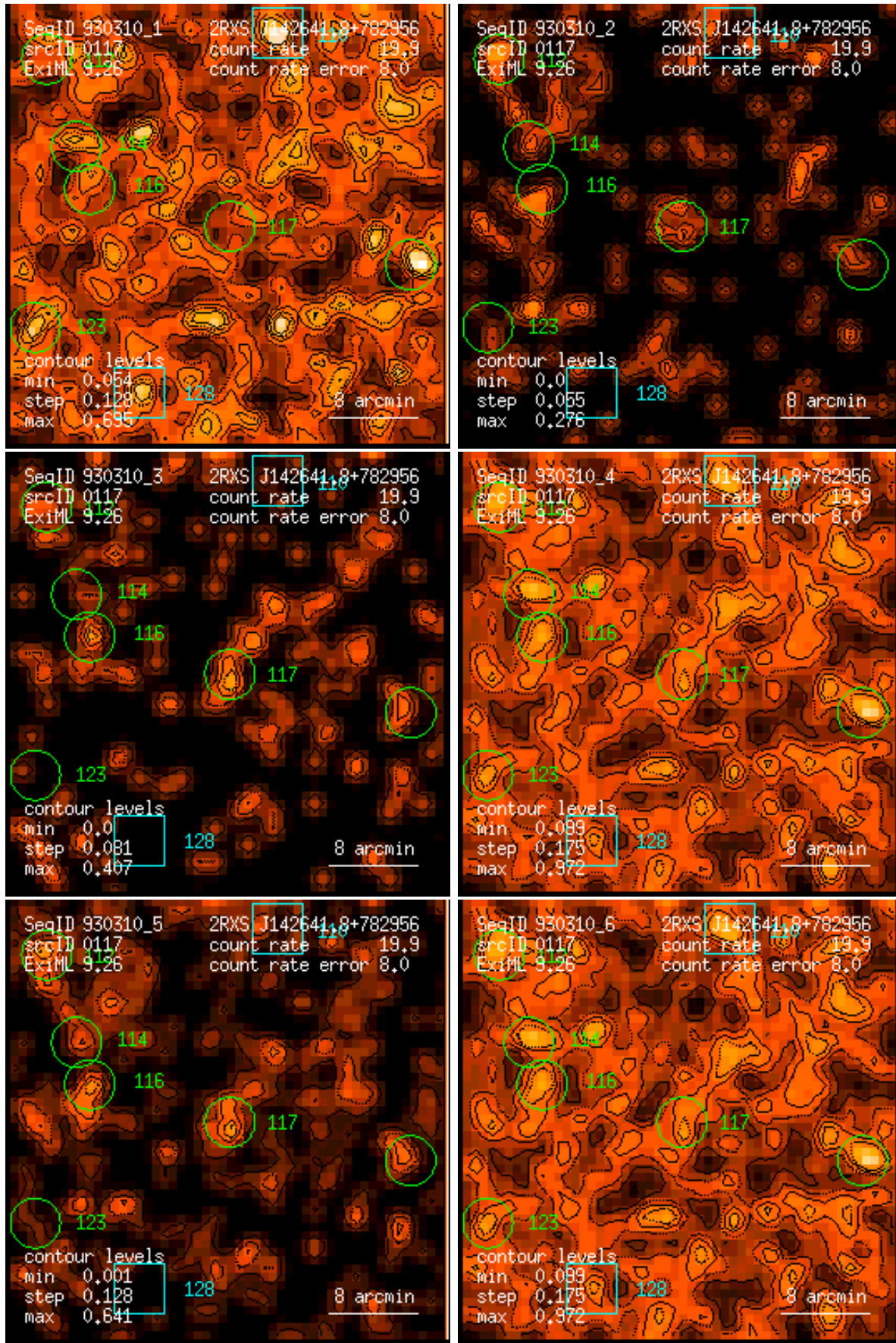
Figure 117: RASS 930310: detection 0117: band rate images, Gaussian filter: (1) PSPC channels 11 – 41, (2) 52 – 90, (3) 91 – 201, (4) 11 – 235, (5) 52 – 201, (6) 11 – 201. Broad band rates in counts/ks. Band rate contour levels in counts/ks/arcmin 2 .
