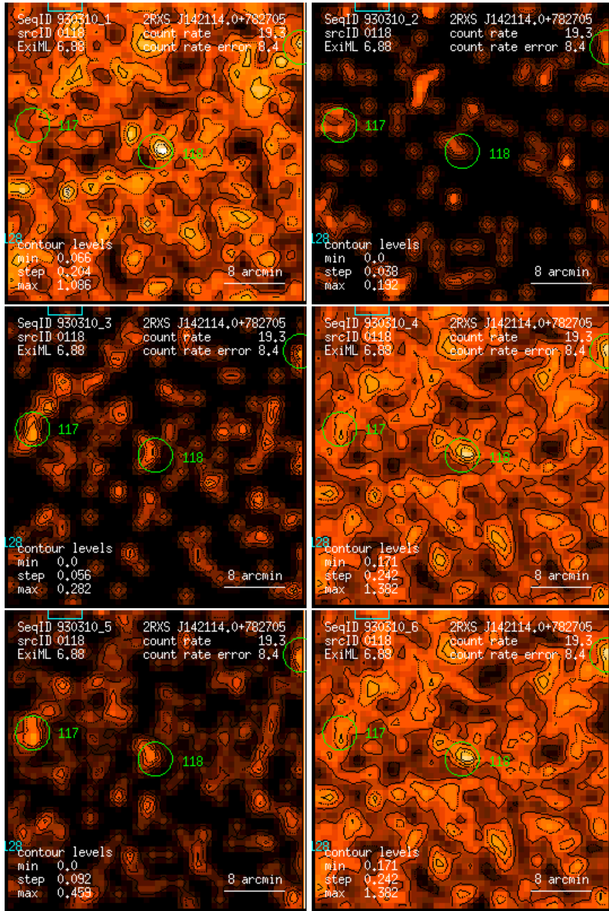
Figure 118: RASS 930310: detection 0118: band rate images, Gaussian filter: (1) PSPC channels 11 – 41, (2) 52 – 90, (3) 91 – 201, (4) 11 – 235, (5) 52 – 201, (6) 11 – 201. Broad band rates in counts/ks. Band rate contour levels in counts/ks/arcmin 2 .
