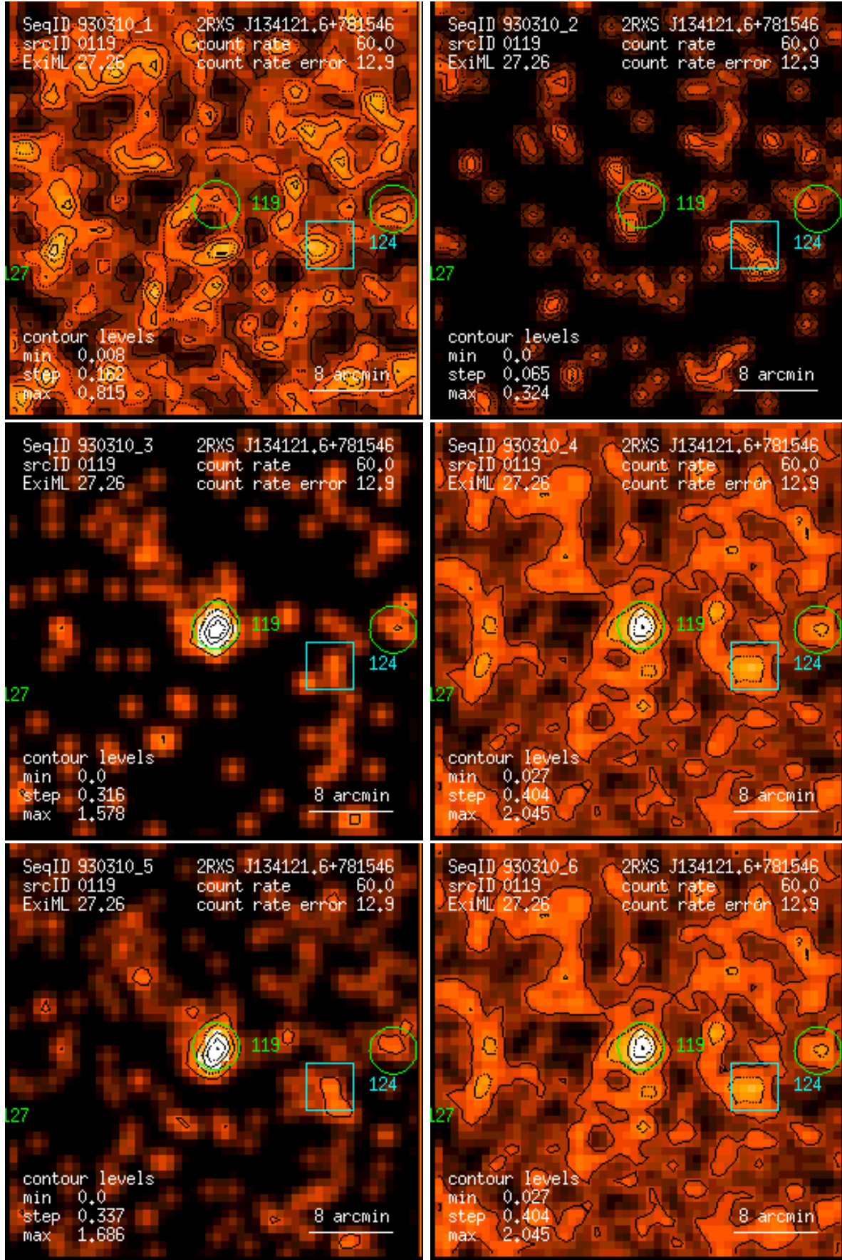
Figure 119: RASS 930310: detection 0119: band rate images, Gaussian filter: (1) PSPC channels 11 – 41, (2) 52 – 90, (3) 91 – 201, (4) 11 – 235, (5) 52 – 201, (6) 11 – 201. Broad band rates in counts/ks. Band rate contour levels in counts/ks/arcmin 2 .
