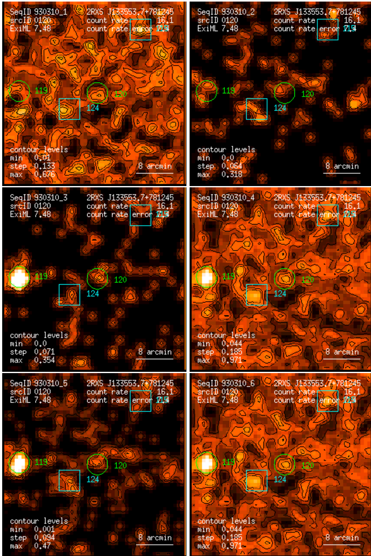
Figure 120: RASS 930310: detection 0120: band rate images, Gaussian filter: (1) PSPC channels 11 – 41, (2) 52 – 90, (3) 91 – 201, (4) 11 – 235, (5) 52 – 201, (6) 11 – 201. Broad band rates in counts/ks. Band rate contour levels in counts/ks/arcmin 2 .
