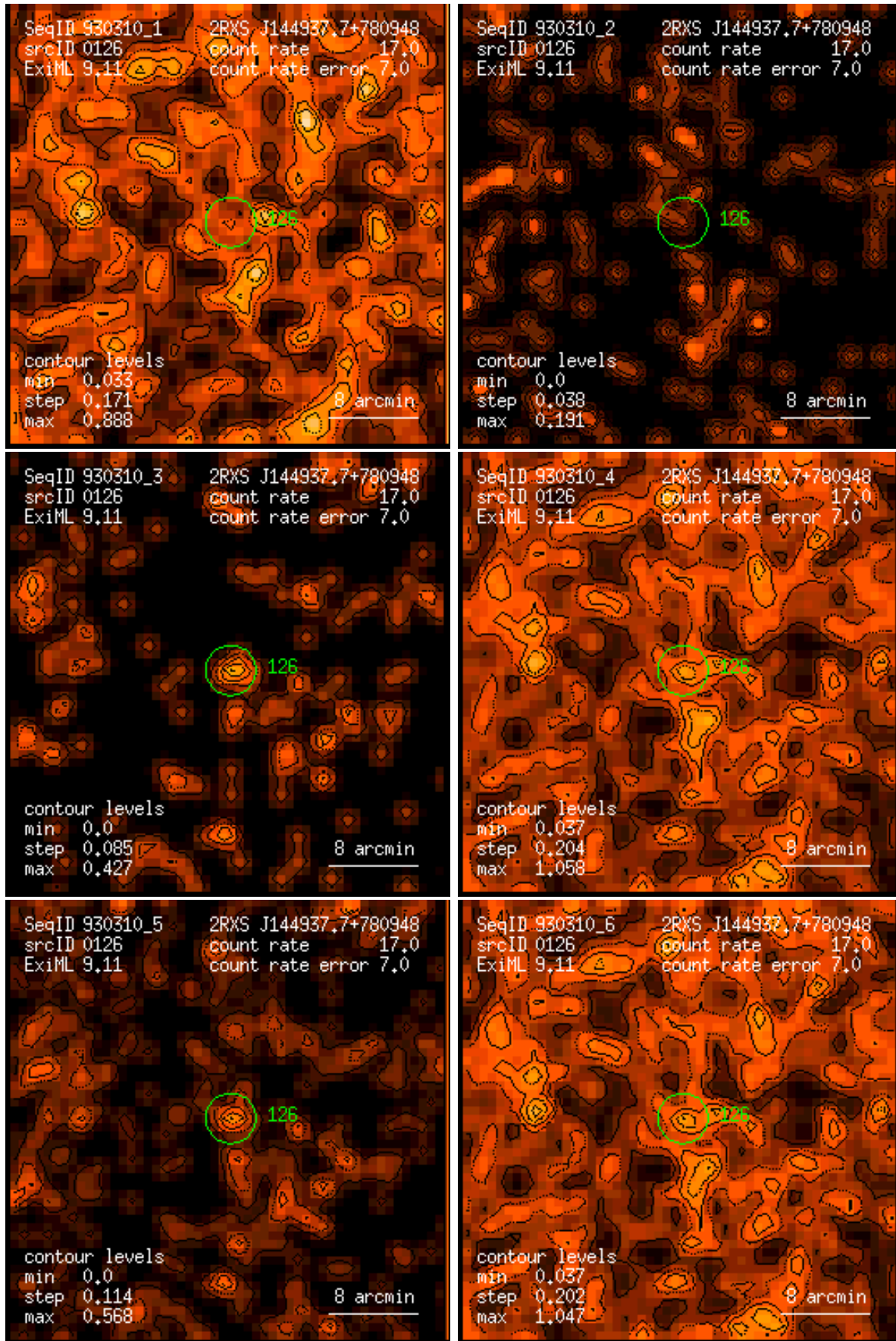
Figure 126: RASS 930310: detection 0126: band rate images, Gaussian filter: (1) PSPC channels 11 – 41, (2) 52 – 90, (3) 91 – 201, (4) 11 – 235, (5) 52 – 201, (6) 11 – 201. Broad band rates in counts/ks. Band rate contour levels in counts/ks/arcmin 2 .
