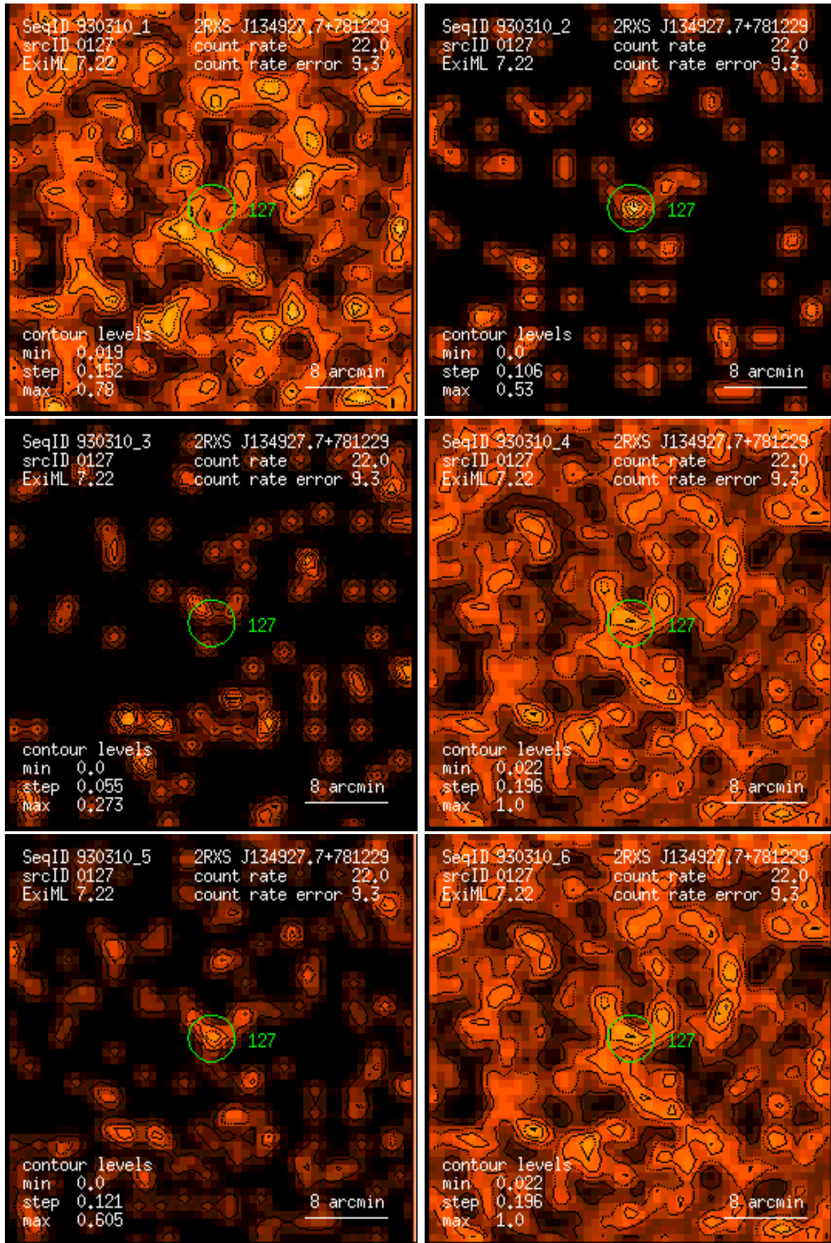
Figure 127: RASS 930310: detection 0127: band rate images, Gaussian filter: (1) PSPC channels 11 – 41, (2) 52 – 90, (3) 91 – 201, (4) 11 – 235, (5) 52 – 201, (6) 11 – 201. Broad band rates in counts/ks. Band rate contour levels in counts/ks/arcmin 2 .
