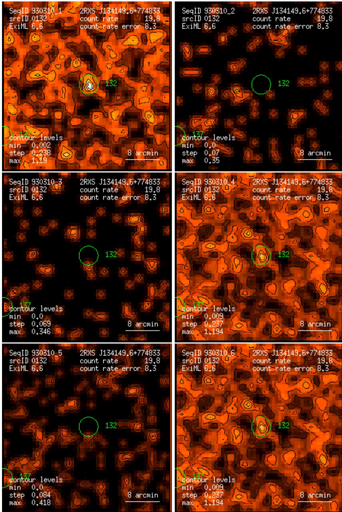
Figure 132: RASS 930310: detection 0132: band rate images, Gaussian filter: (1) PSPC channels 11 – 41, (2) 52 – 90, (3) 91 – 201, (4) 11 – 235, (5) 52 – 201, (6) 11 – 201. Broad band rates in counts/ks. Band rate contour levels in counts/ks/arcmin 2 .
