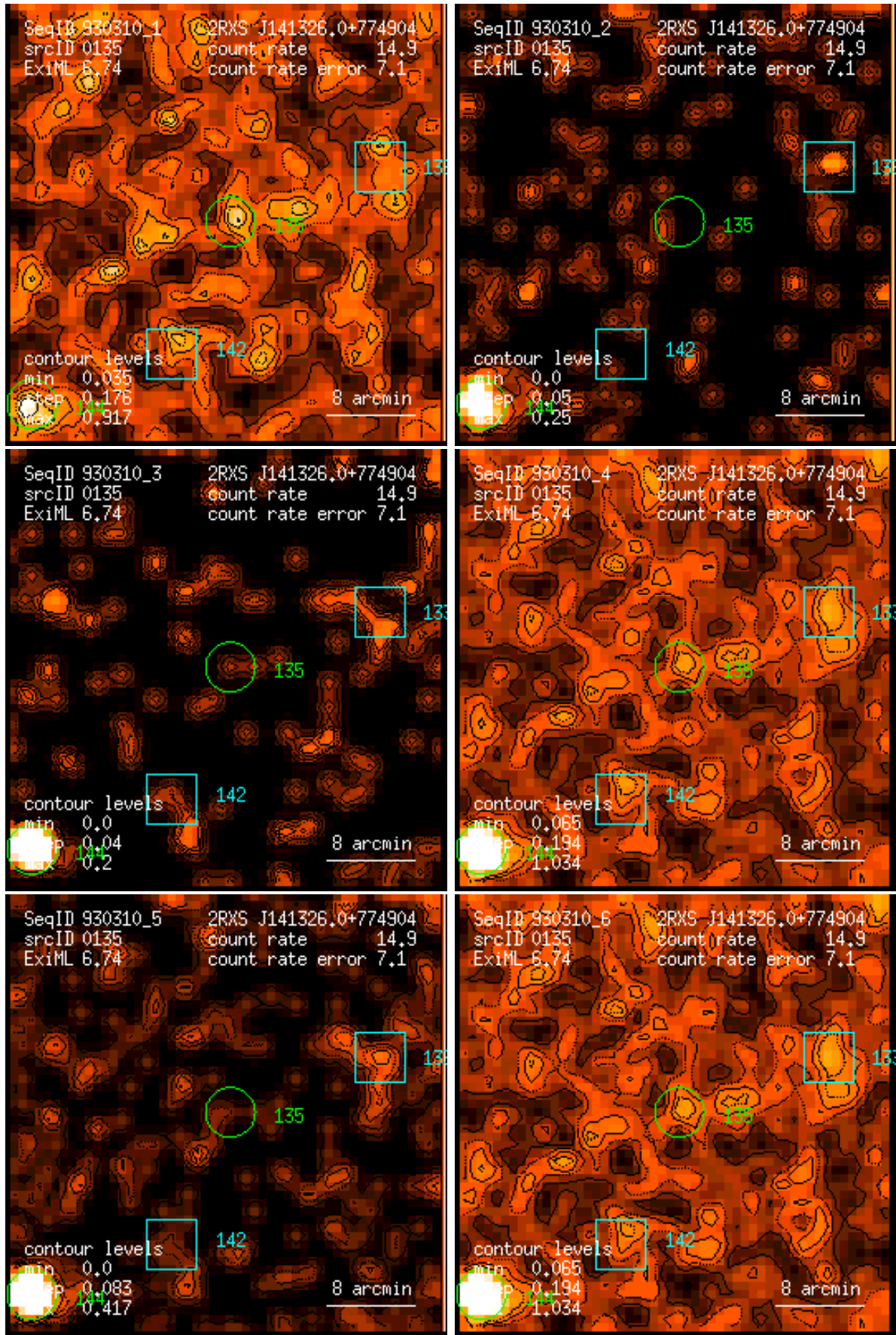
Figure 135: RASS 930310: detection 0135: band rate images, Gaussian filter: (1) PSPC channels 11 – 41, (2) 52 – 90, (3) 91 – 201, (4) 11 – 235, (5) 52 – 201, (6) 11 – 201. Broad band rates in counts/ks. Band rate contour levels in counts/ks/arcmin 2 .
