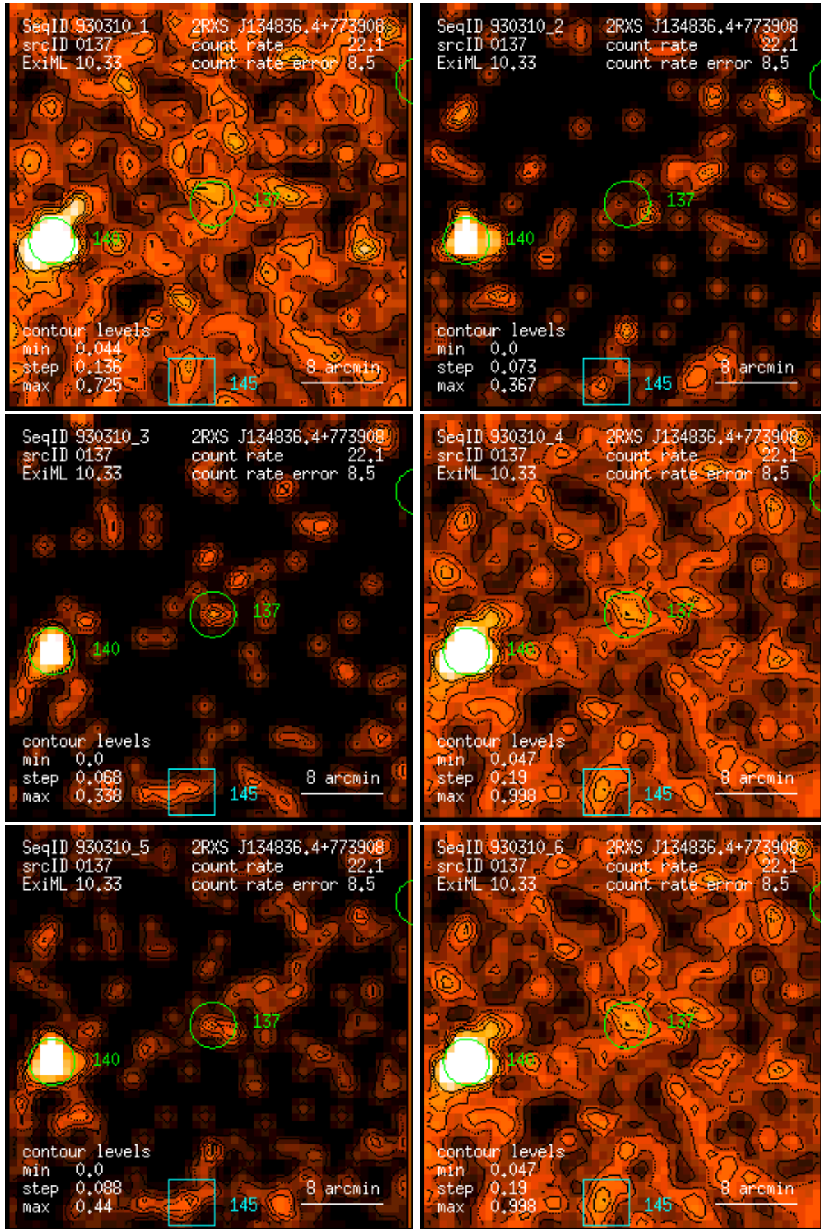
Figure 137: RASS 930310: detection 0137: band rate images, Gaussian filter: (1) PSPC channels 11 – 41, (2) 52 – 90, (3) 91 – 201, (4) 11 – 235, (5) 52 – 201, (6) 11 – 201. Broad band rates in counts/ks. Band rate contour levels in counts/ks/arcmin 2 .
