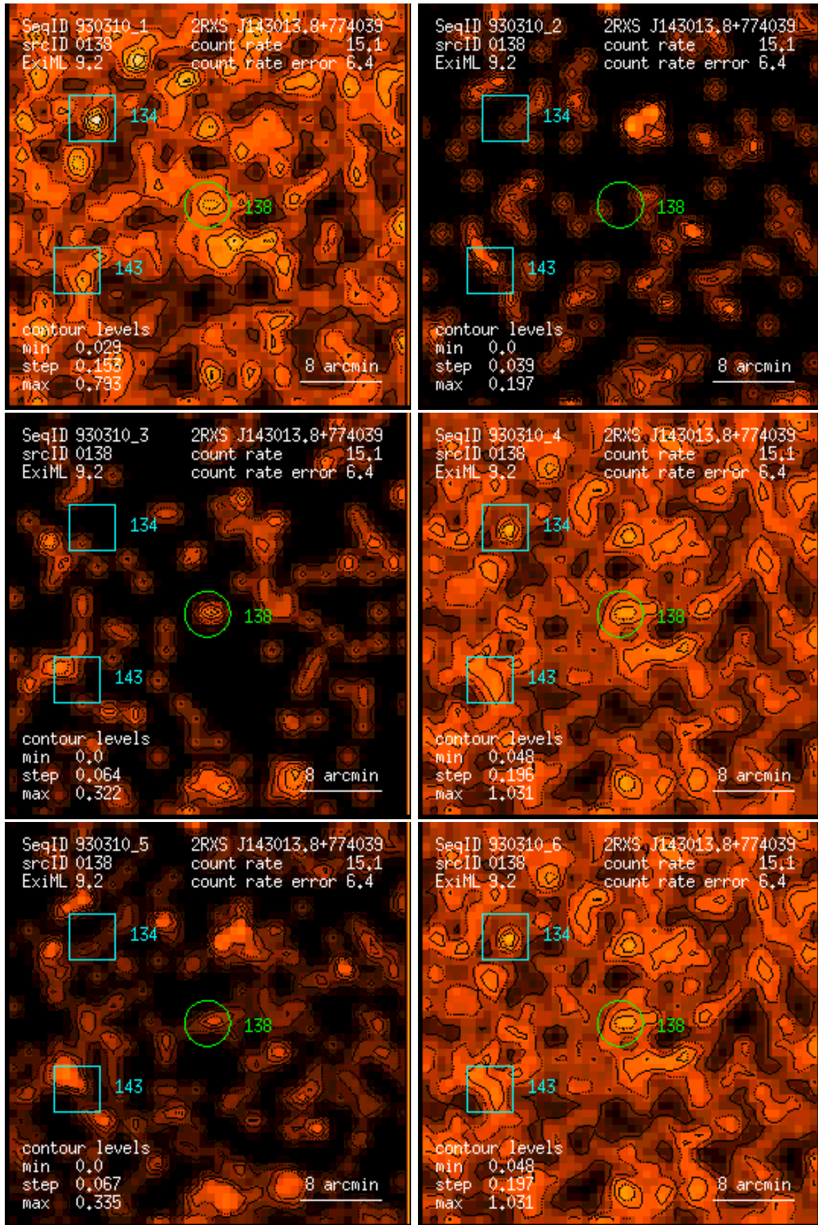
Figure 138: RASS 930310: detection 0138: band rate images, Gaussian filter: (1) PSPC channels 11 – 41, (2) 52 – 90, (3) 91 – 201, (4) 11 – 235, (5) 52 – 201, (6) 11 – 201. Broad band rates in counts/ks. Band rate contour levels in counts/ks/arcmin 2 .
