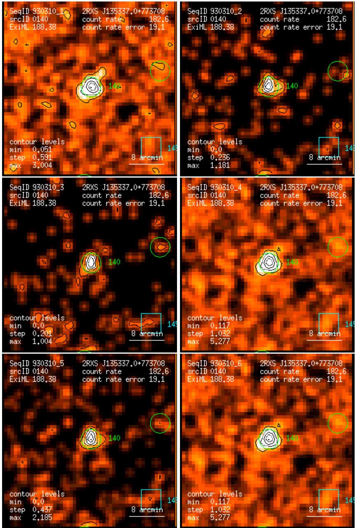
Figure 140: RASS 930310: detection 0140: band rate images, Gaussian filter: (1) PSPC channels 11 – 41, (2) 52 – 90, (3) 91 – 201, (4) 11 – 235, (5) 52 – 201, (6) 11 – 201. Broad band rates in counts/ks. Band rate contour levels in counts/ks/arcmin 2 .
