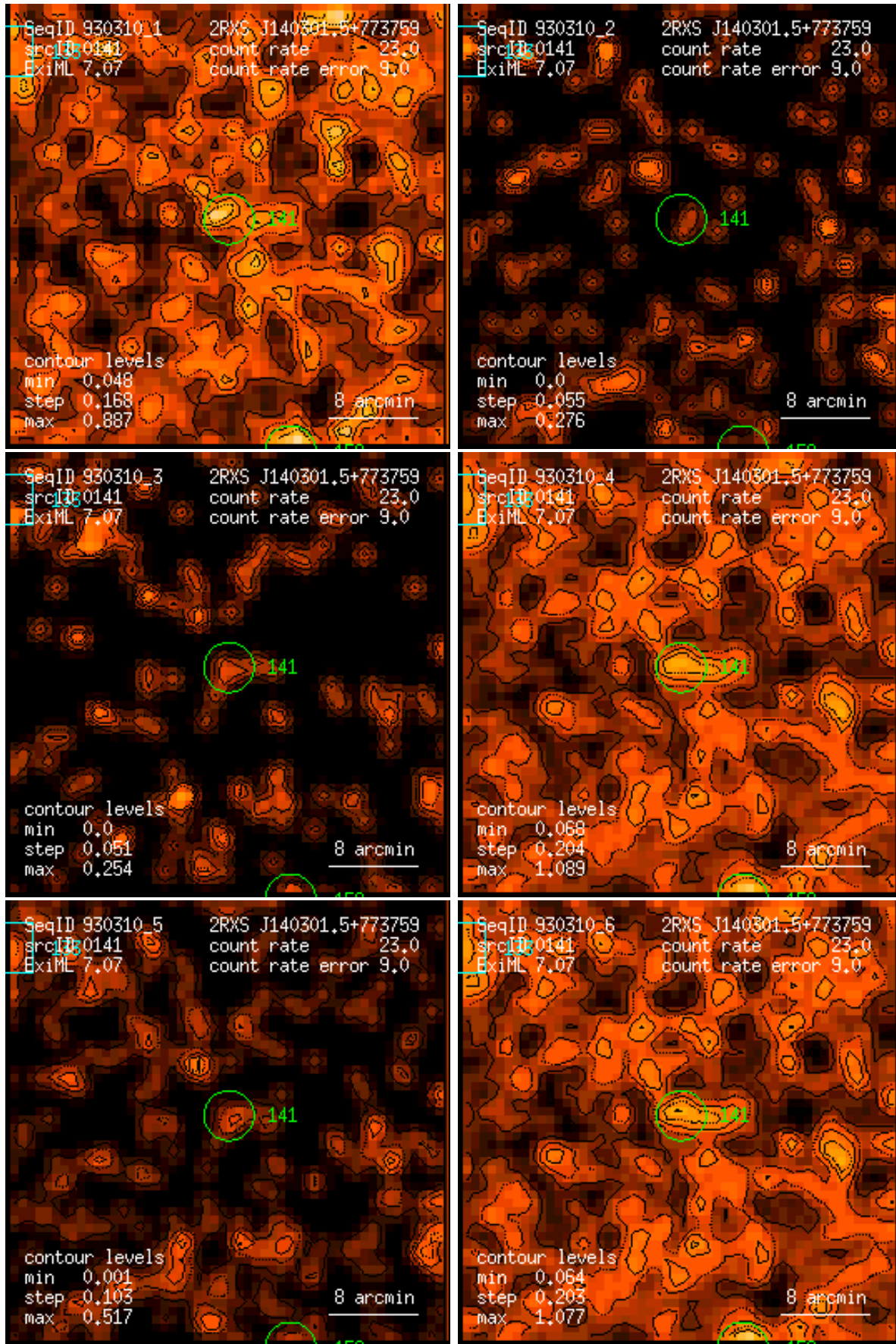
Figure 141: RASS 930310: detection 0141: band rate images, Gaussian filter: (1) PSPC channels 11 – 41, (2) 52 – 90, (3) 91 – 201, (4) 11 – 235, (5) 52 – 201, (6) 11 – 201. Broad band rates in counts/ks. Band rate contour levels in counts/ks/arcmin 2 .
