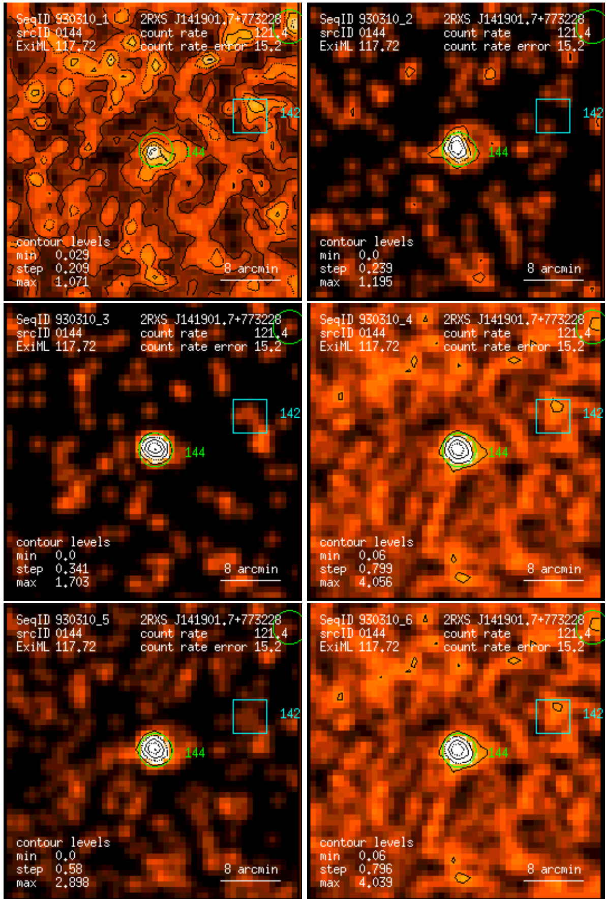
Figure 144: RASS 930310: detection 0144: band rate images, Gaussian filter: (1) PSPC channels 11 – 41, (2) 52 – 90, (3) 91 – 201, (4) 11 – 235, (5) 52 – 201, (6) 11 – 201. Broad band rates in counts/ks. Band rate contour levels in counts/ks/arcmin 2 .
