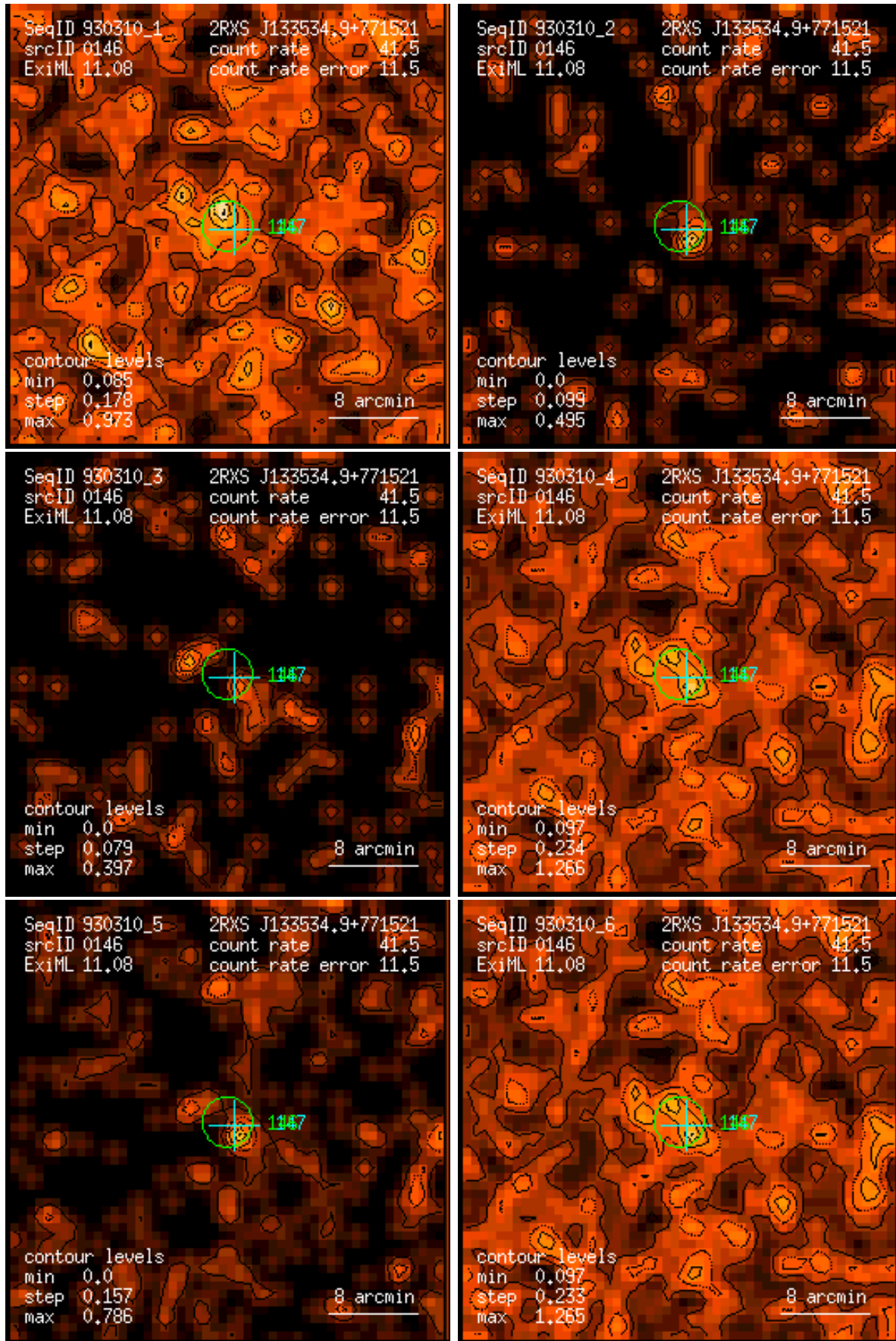
Figure 146: RASS 930310: detection 0146: band rate images, Gaussian filter: (1) PSPC channels 11 – 41, (2) 52 – 90, (3) 91 – 201, (4) 11 – 235, (5) 52 – 201, (6) 11 – 201. Broad band rates in counts/ks. Band rate contour levels in counts/ks/arcmin 2 .
