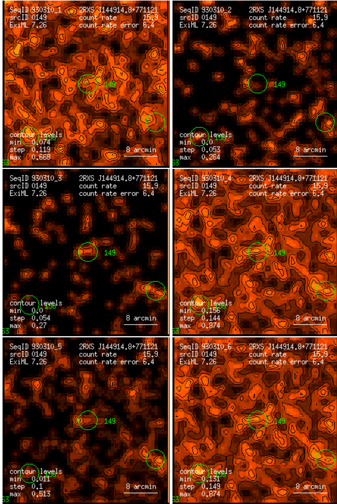
Figure 149: RASS 930310: detection 0149: band rate images, Gaussian filter: (1) PSPC channels 11 – 41, (2) 52 – 90, (3) 91 – 201, (4) 11 – 235, (5) 52 – 201, (6) 11 – 201. Broad band rates in counts/ks. Band rate contour levels in counts/ks/arcmin 2 .
