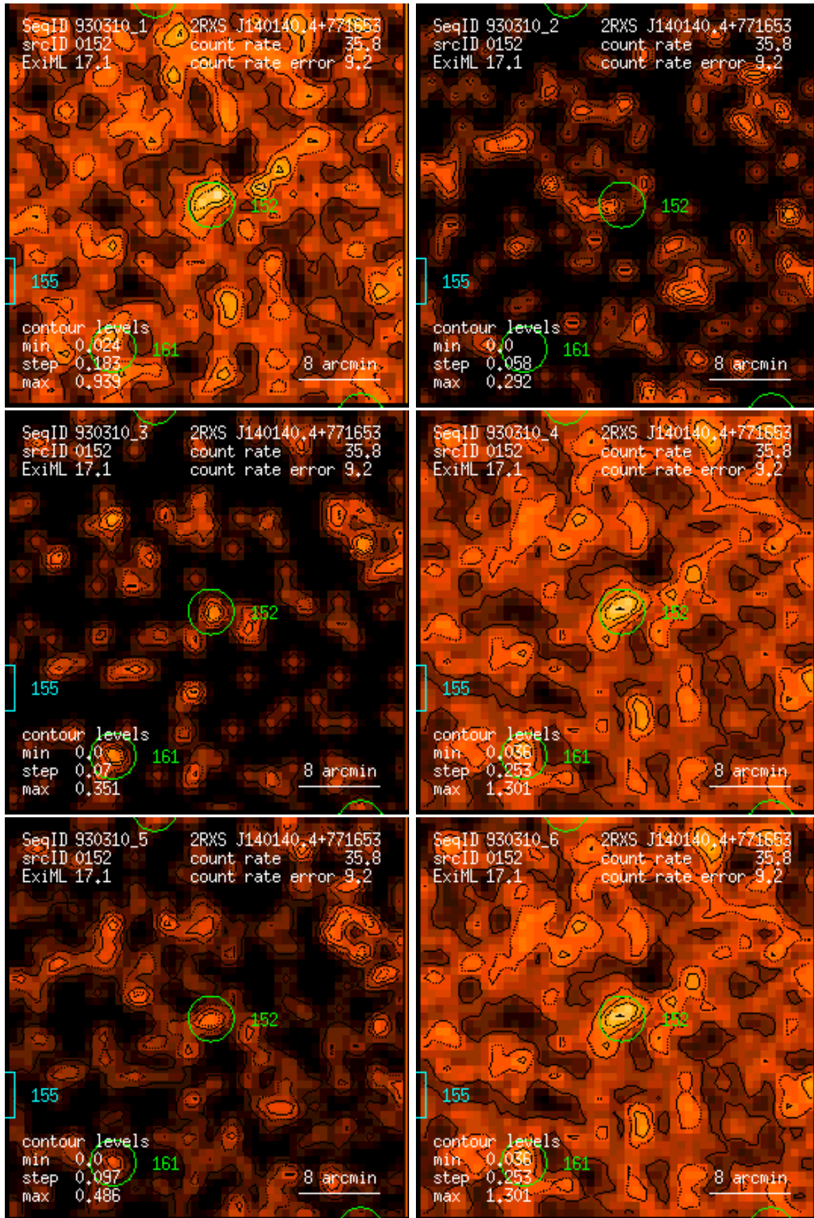
Figure 152: RASS 930310: detection 0152: band rate images, Gaussian filter: (1) PSPC channels 11 – 41, (2) 52 – 90, (3) 91 – 201, (4) 11 – 235, (5) 52 – 201, (6) 11 – 201. Broad band rates in counts/ks. Band rate contour levels in counts/ks/arcmin 2 .
