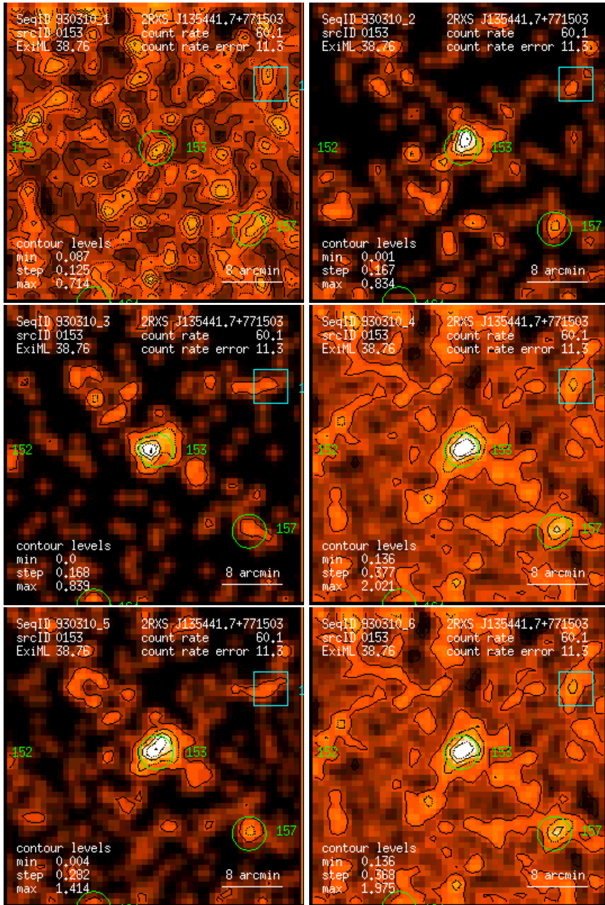
Figure 153: RASS 930310: detection 0153: band rate images, Gaussian filter: (1) PSPC channels 11 – 41, (2) 52 – 90, (3) 91 – 201, (4) 11 – 235, (5) 52 – 201, (6) 11 – 201. Broad band rates in counts/ks. Band rate contour levels in counts/ks/arcmin 2 .
