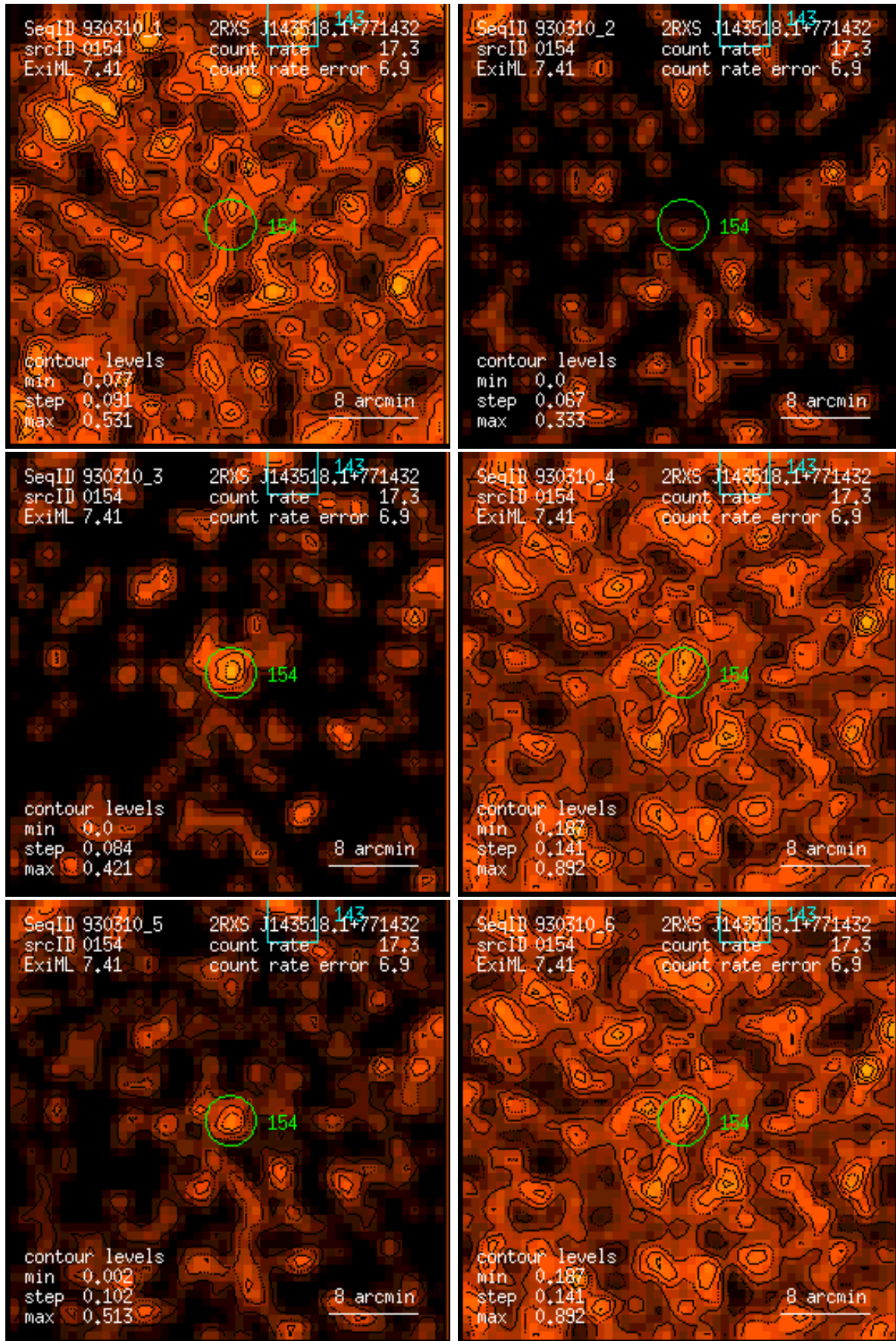
Figure 154: RASS 930310: detection 0154: band rate images, Gaussian filter: (1) PSPC channels 11 – 41, (2) 52 – 90, (3) 91 – 201, (4) 11 – 235, (5) 52 – 201, (6) 11 – 201. Broad band rates in counts/ks. Band rate contour levels in counts/ks/arcmin 2 .
