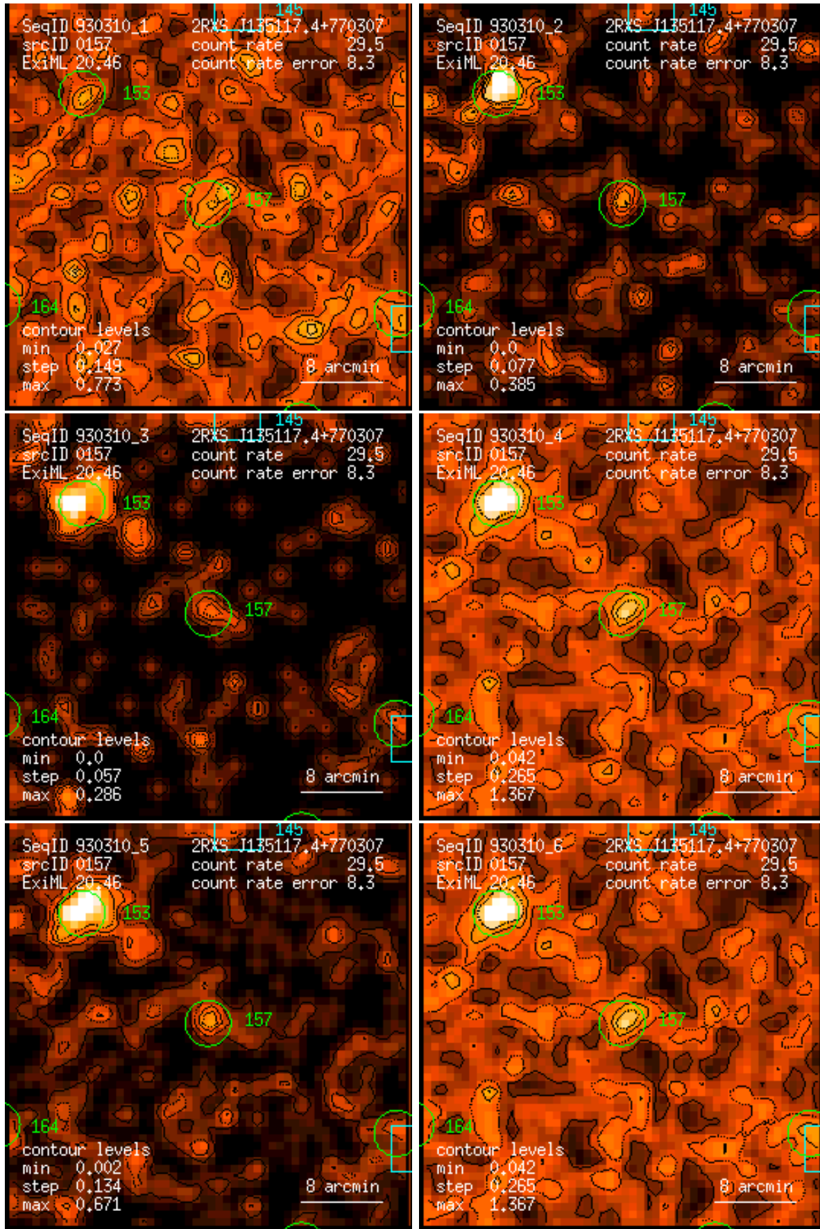
Figure 157: RASS 930310: detection 0157: band rate images, Gaussian filter: (1) PSPC channels 11 – 41, (2) 52 – 90, (3) 91 – 201, (4) 11 – 235, (5) 52 – 201, (6) 11 – 201. Broad band rates in counts/ks. Band rate contour levels in counts/ks/arcmin 2 .
