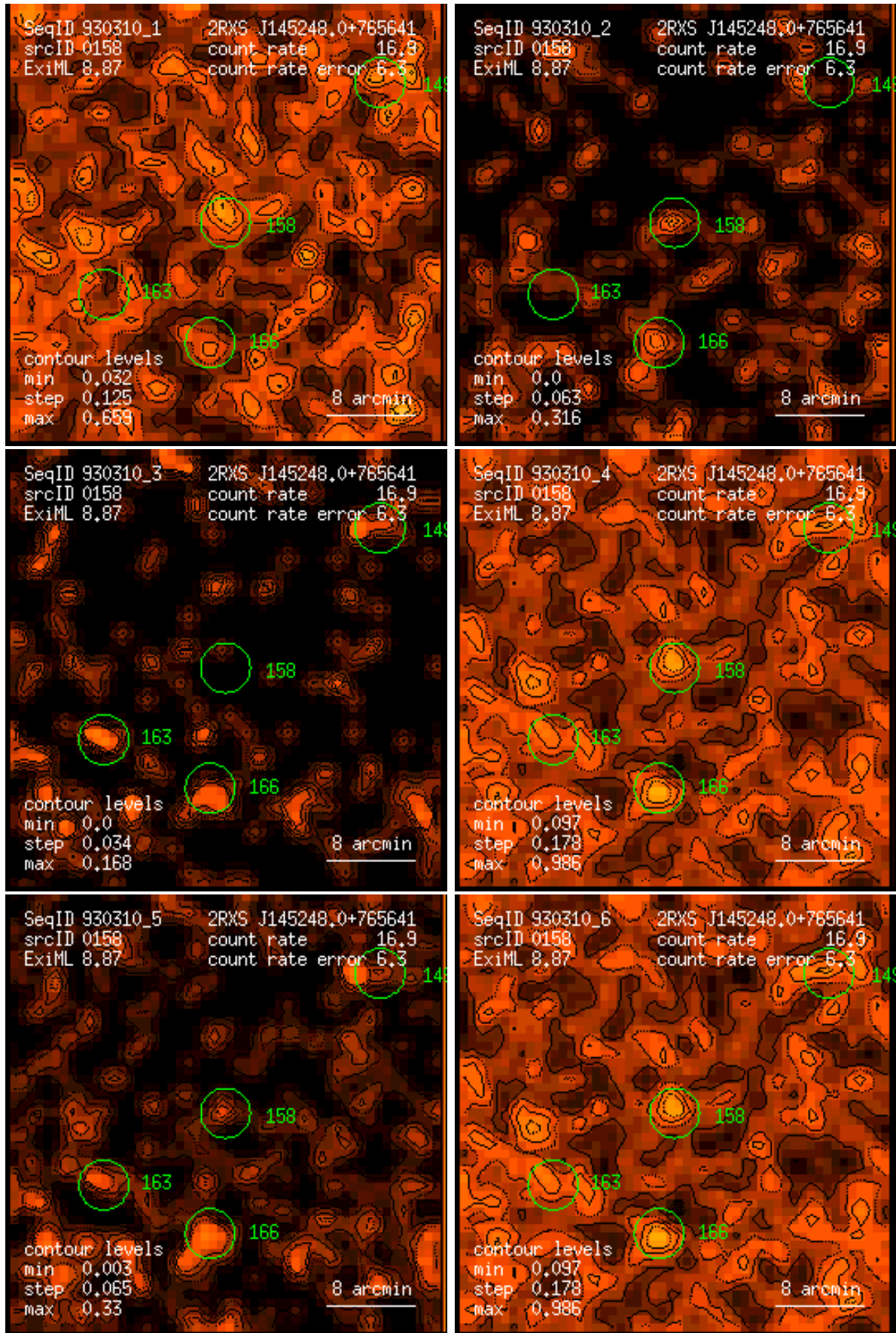
Figure 158: RASS 930310: detection 0158: band rate images, Gaussian filter: (1) PSPC channels 11 – 41, (2) 52 – 90, (3) 91 – 201, (4) 11 – 235, (5) 52 – 201, (6) 11 – 201. Broad band rates in counts/ks. Band rate contour levels in counts/ks/arcmin 2 .
