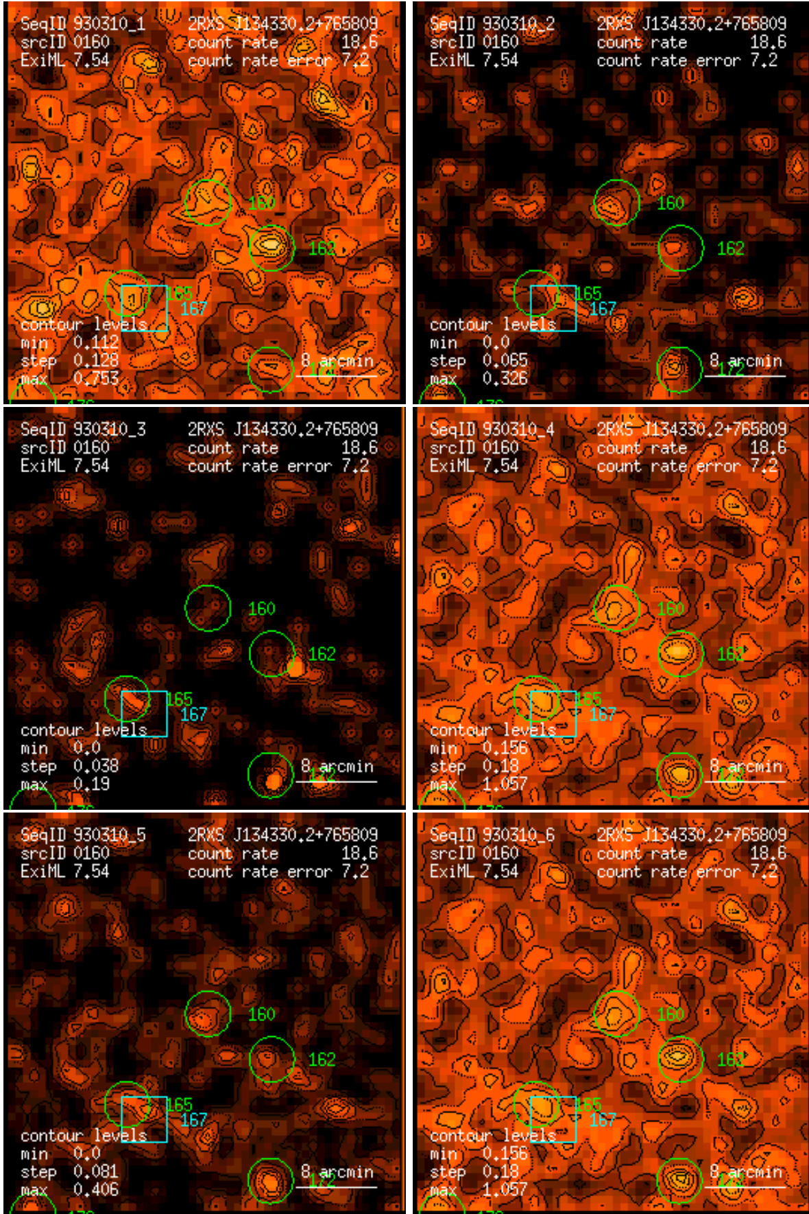
Figure 160: RASS 930310: detection 0160: band rate images, Gaussian filter: (1) PSPC channels 11 – 41, (2) 52 – 90, (3) 91 – 201, (4) 11 – 235, (5) 52 – 201, (6) 11 – 201. Broad band rates in counts/ks. Band rate contour levels in counts/ks/arcmin 2 .
