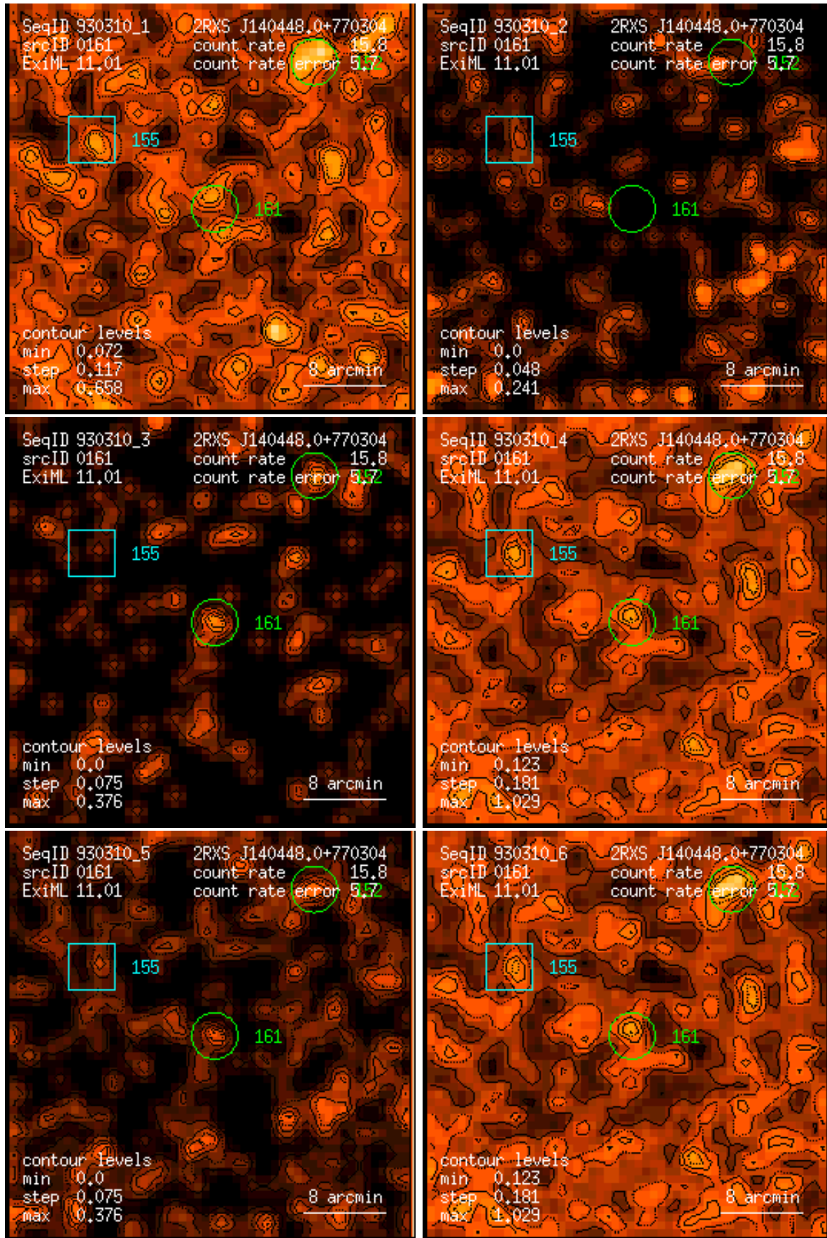
Figure 161: RASS 930310: detection 0161: band rate images, Gaussian filter: (1) PSPC channels 11 – 41, (2) 52 – 90, (3) 91 – 201, (4) 11 – 235, (5) 52 – 201, (6) 11 – 201. Broad band rates in counts/ks. Band rate contour levels in counts/ks/arcmin 2 .
