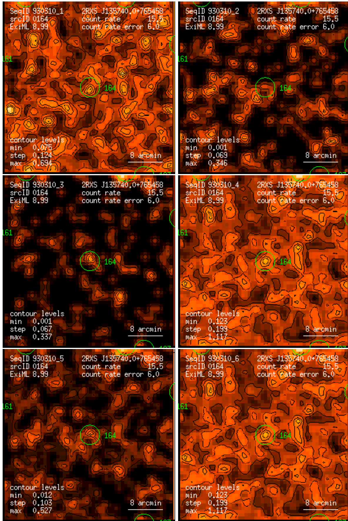
Figure 164: RASS 930310: detection 0164: band rate images, Gaussian filter: (1) PSPC channels 11 – 41, (2) 52 – 90, (3) 91 – 201, (4) 11 – 235, (5) 52 – 201, (6) 11 – 201. Broad band rates in counts/ks. Band rate contour levels in counts/ks/arcmin 2 .
