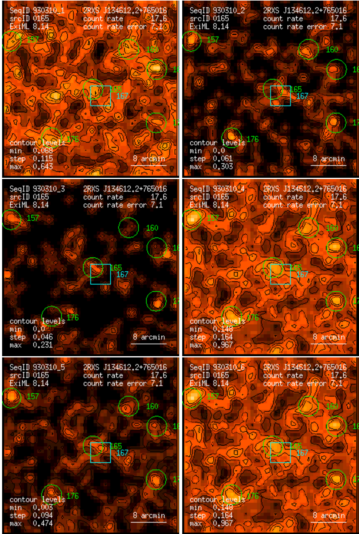
Figure 165: RASS 930310: detection 0165: band rate images, Gaussian filter: (1) PSPC channels 11 – 41, (2) 52 – 90, (3) 91 – 201, (4) 11 – 235, (5) 52 – 201, (6) 11 – 201. Broad band rates in counts/ks. Band rate contour levels in counts/ks/arcmin 2 .
