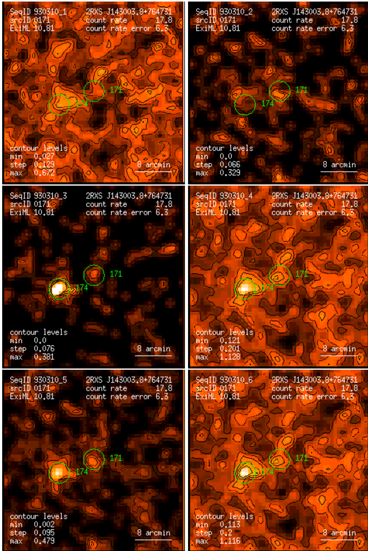
Figure 171: RASS 930310: detection 0171: band rate images, Gaussian filter: (1) PSPC channels 11 – 41, (2) 52 – 90, (3) 91 – 201, (4) 11 – 235, (5) 52 – 201, (6) 11 – 201. Broad band rates in counts/ks. Band rate contour levels in counts/ks/arcmin 2 .
