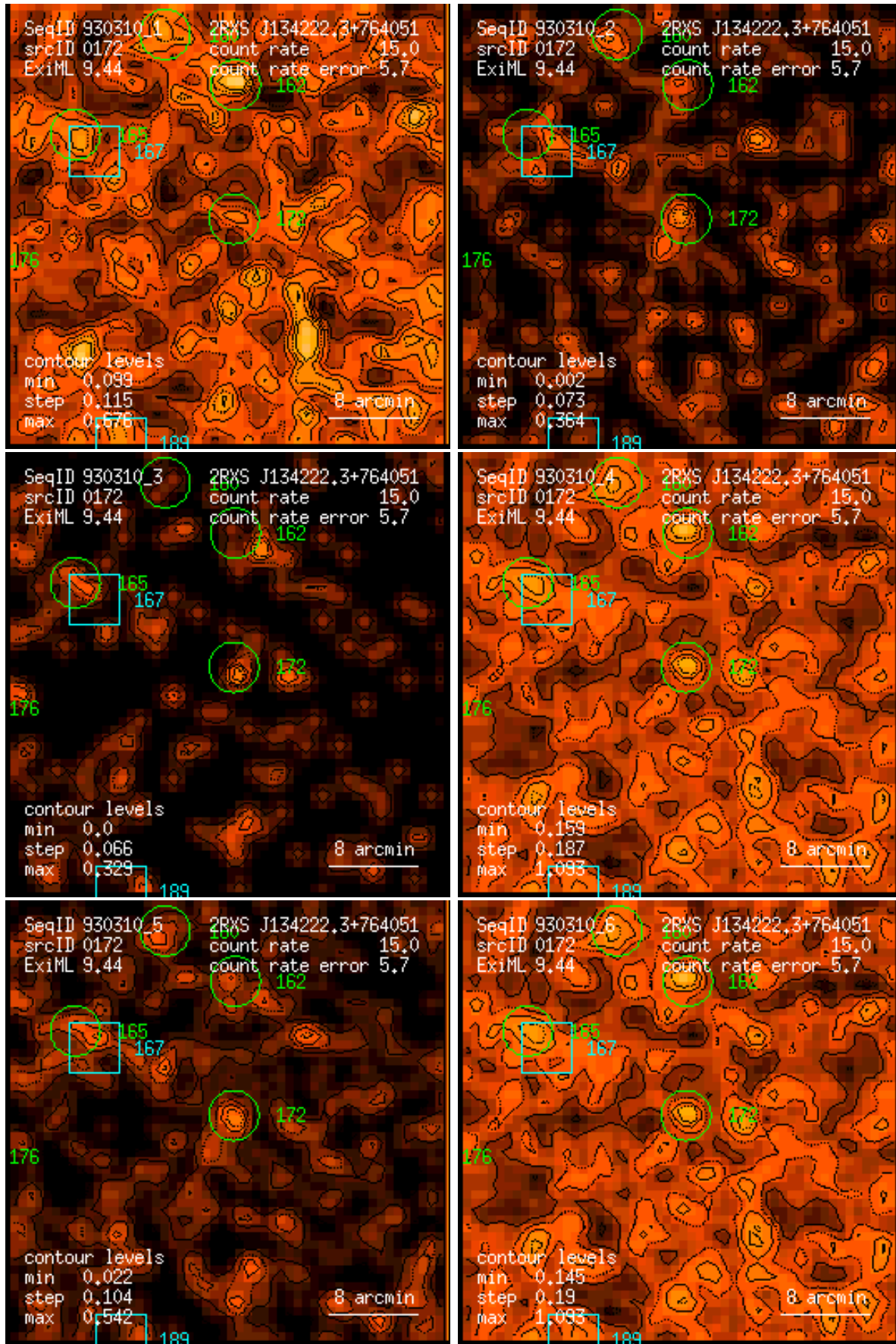
Figure 172: RASS 930310: detection 0172: band rate images, Gaussian filter: (1) PSPC channels 11 – 41, (2) 52 – 90, (3) 91 – 201, (4) 11 – 235, (5) 52 – 201, (6) 11 – 201. Broad band rates in counts/ks. Band rate contour levels in counts/ks/arcmin 2 .
