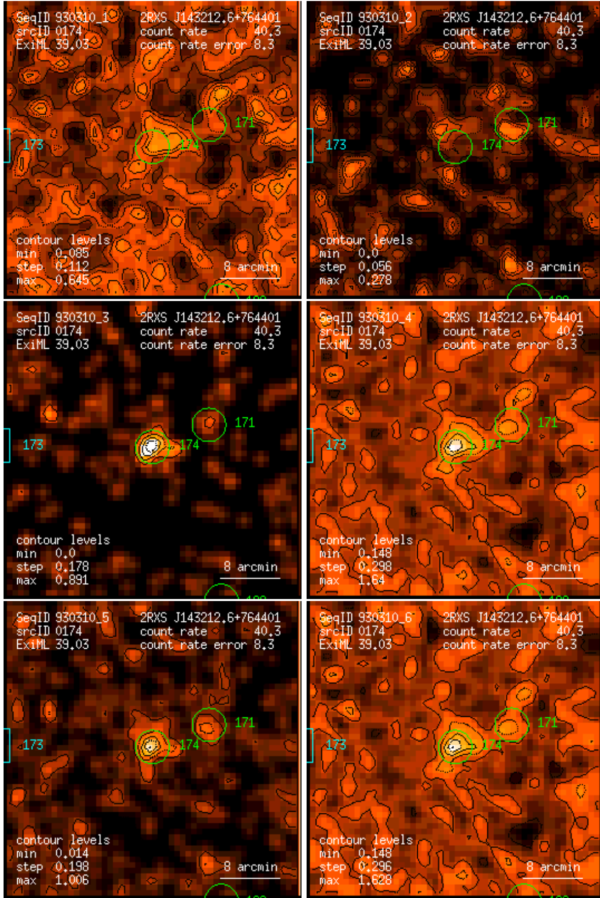
Figure 174: RASS 930310: detection 0174: band rate images, Gaussian filter: (1) PSPC channels 11 – 41, (2) 52 – 90, (3) 91 – 201, (4) 11 – 235, (5) 52 – 201, (6) 11 – 201. Broad band rates in counts/ks. Band rate contour levels in counts/ks/arcmin 2 .
