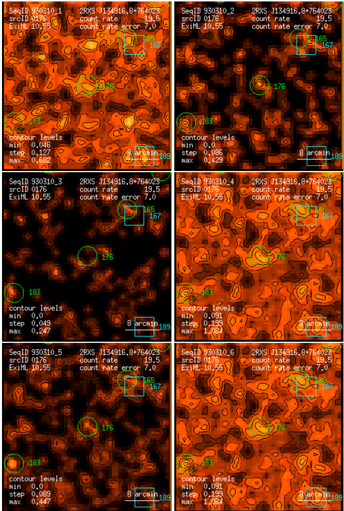
Figure 176: RASS 930310: detection 0176: band rate images, Gaussian filter: (1) PSPC channels 11 – 41, (2) 52 – 90, (3) 91 – 201, (4) 11 – 235, (5) 52 – 201, (6) 11 – 201. Broad band rates in counts/ks. Band rate contour levels in counts/ks/arcmin 2 .
