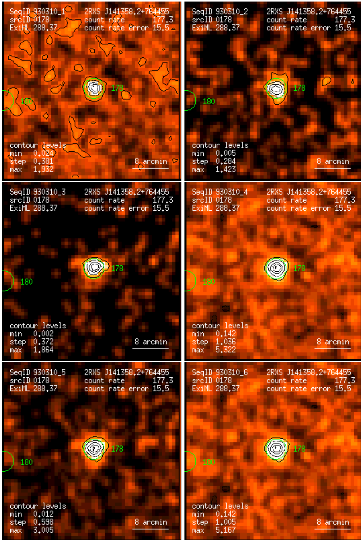
Figure 178: RASS 930310: detection 0178: band rate images, Gaussian filter: (1) PSPC channels 11 – 41, (2) 52 – 90, (3) 91 – 201, (4) 11 – 235, (5) 52 – 201, (6) 11 – 201. Broad band rates in counts/ks. Band rate contour levels in counts/ks/arcmin 2 .
