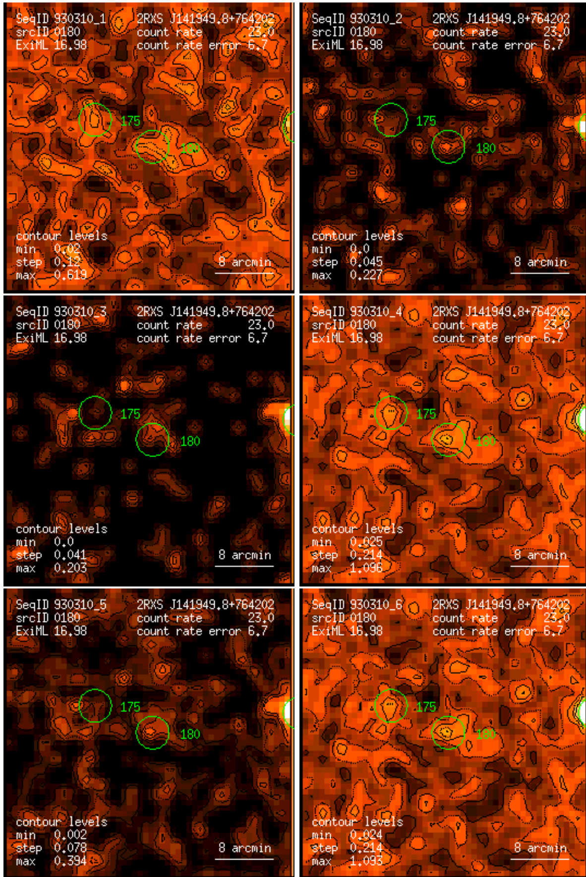
Figure 180: RASS 930310: detection 0180: band rate images, Gaussian filter: (1) PSPC channels 11 – 41, (2) 52 – 90, (3) 91 – 201, (4) 11 – 235, (5) 52 – 201, (6) 11 – 201. Broad band rates in counts/ks. Band rate contour levels in counts/ks/arcmin 2 .
