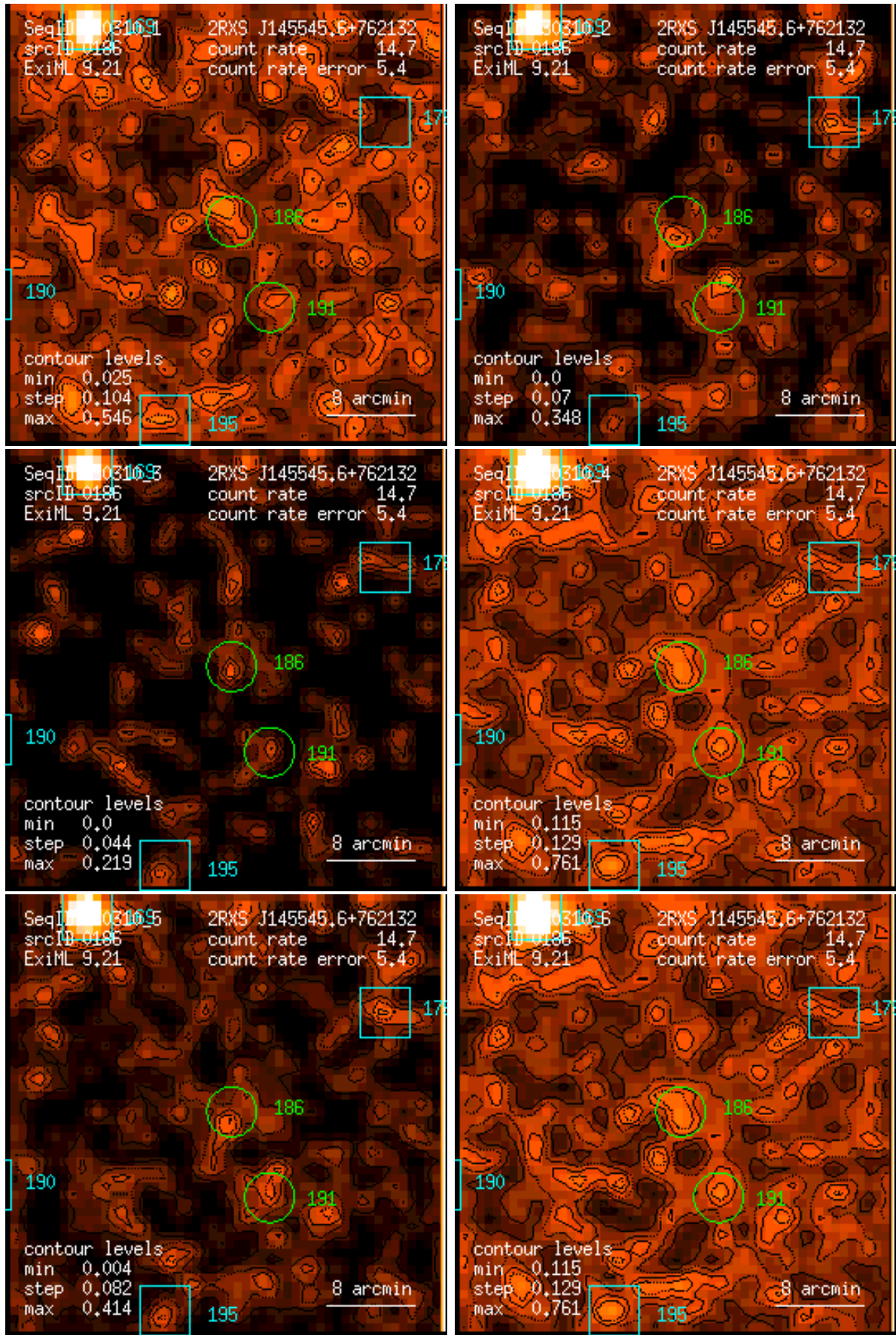
Figure 186: RASS 930310: detection 0186: band rate images, Gaussian filter: (1) PSPC channels 11 – 41, (2) 52 – 90, (3) 91 – 201, (4) 11 – 235, (5) 52 – 201, (6) 11 – 201. Broad band rates in counts/ks. Band rate contour levels in counts/ks/arcmin 2 .
