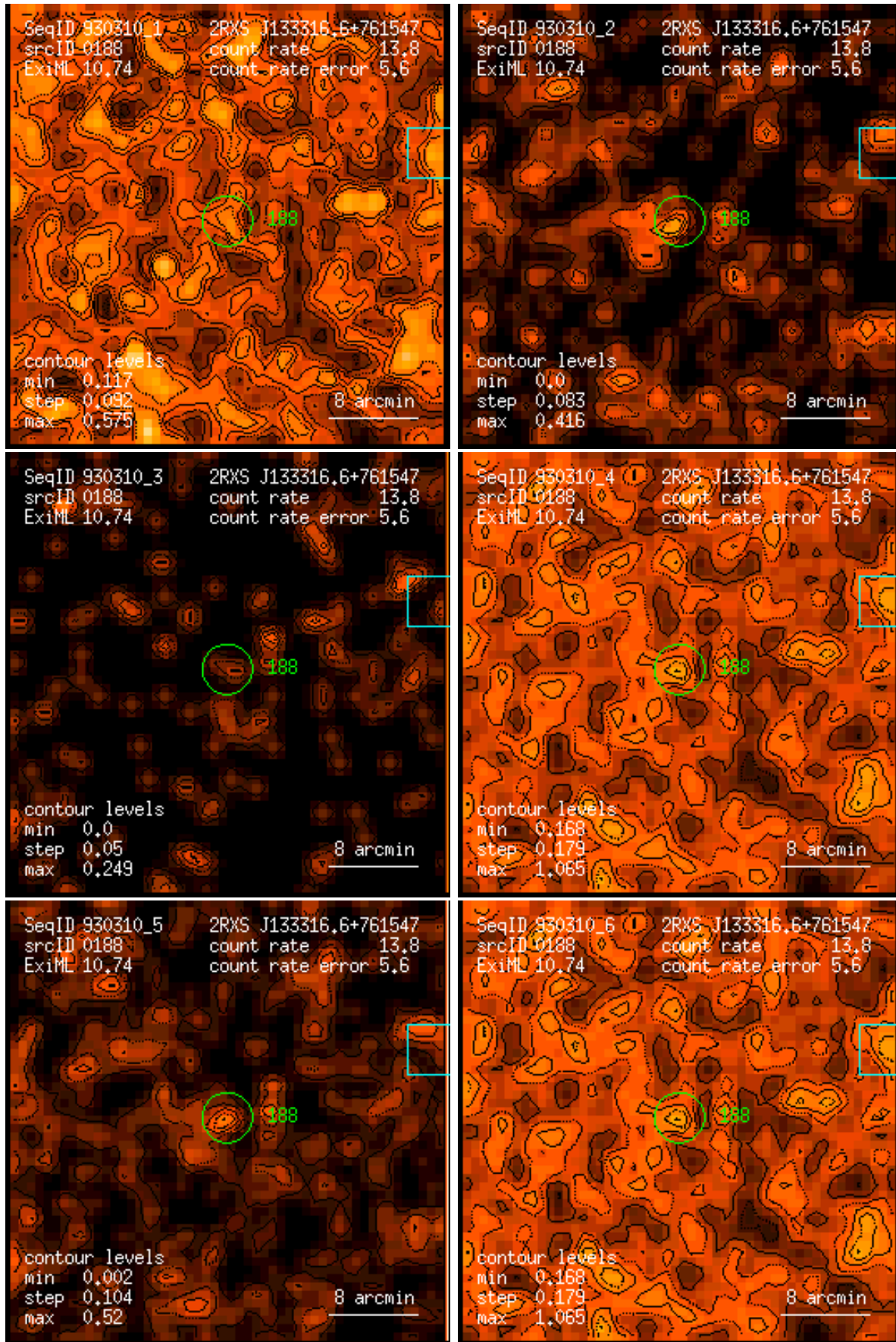
Figure 188: RASS 930310: detection 0188: band rate images, Gaussian filter: (1) PSPC channels 11 – 41, (2) 52 – 90, (3) 91 – 201, (4) 11 – 235, (5) 52 – 201, (6) 11 – 201. Broad band rates in counts/ks. Band rate contour levels in counts/ks/arcmin 2 .
