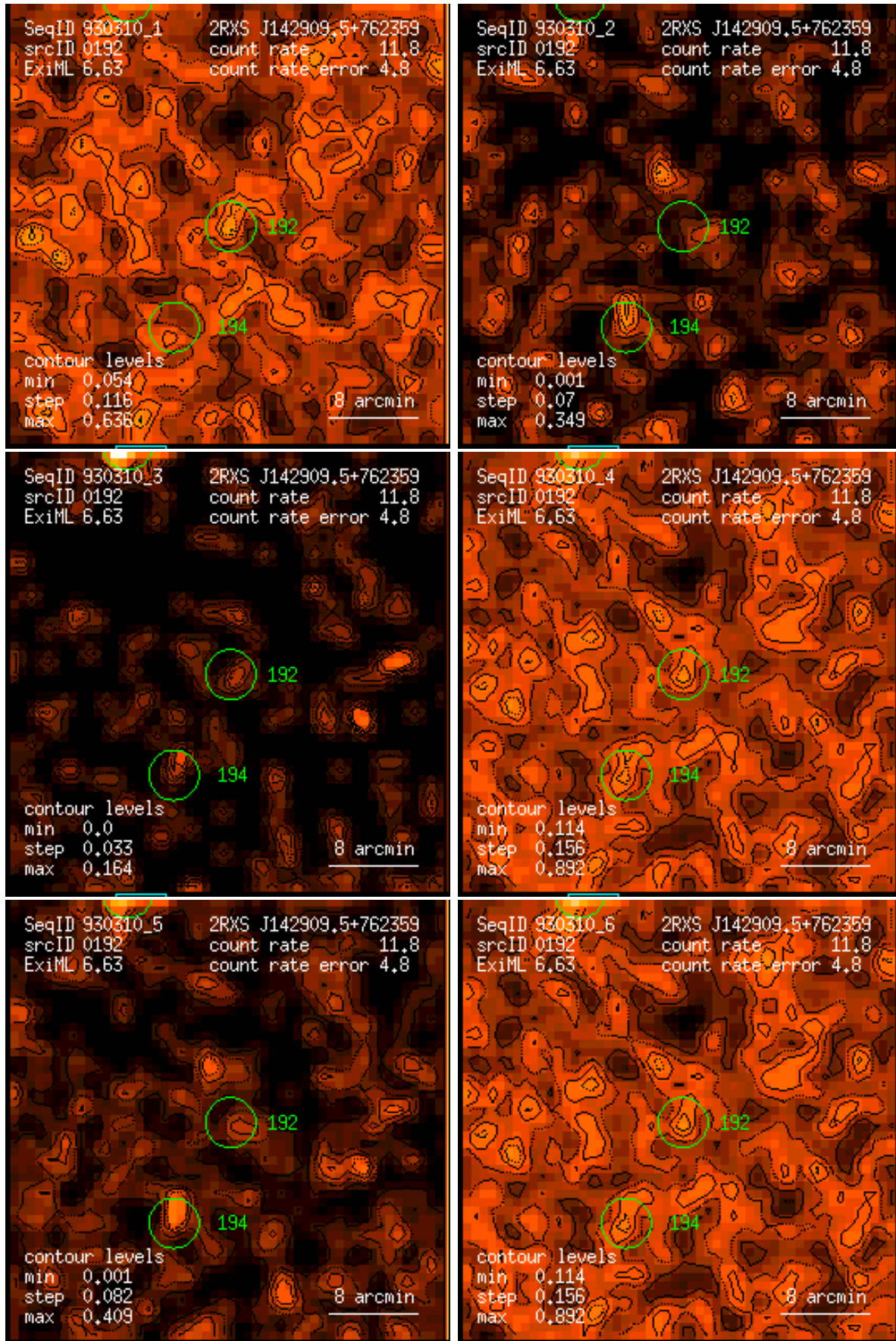
Figure 192: RASS 930310: detection 0192: band rate images, Gaussian filter: (1) PSPC channels 11 – 41, (2) 52 – 90, (3) 91 – 201, (4) 11 – 235, (5) 52 – 201, (6) 11 – 201. Broad band rates in counts/ks. Band rate contour levels in counts/ks/arcmin 2 .
