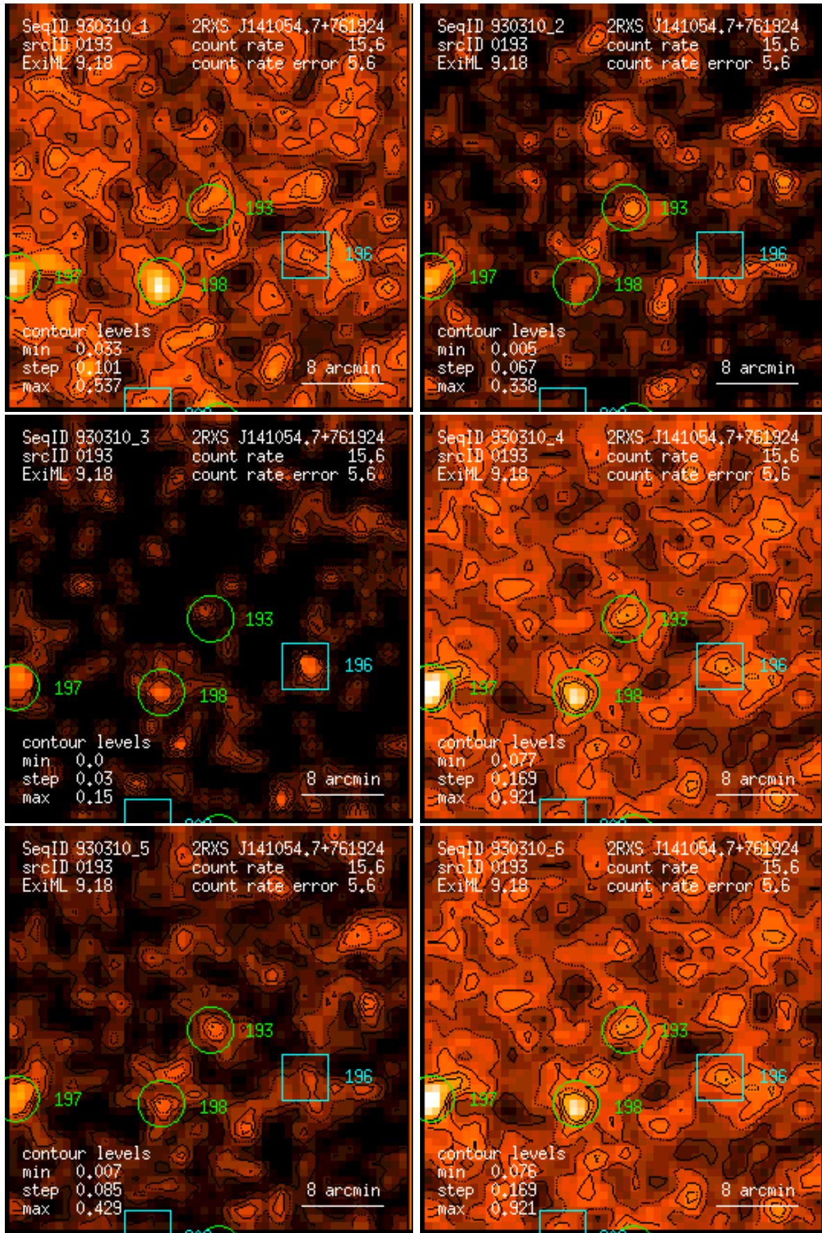
Figure 193: RASS 930310: detection 0193: band rate images, Gaussian filter: (1) PSPC channels 11 – 41, (2) 52 – 90, (3) 91 – 201, (4) 11 – 235, (5) 52 – 201, (6) 11 – 201. Broad band rates in counts/ks. Band rate contour levels in counts/ks/arcmin 2 .
