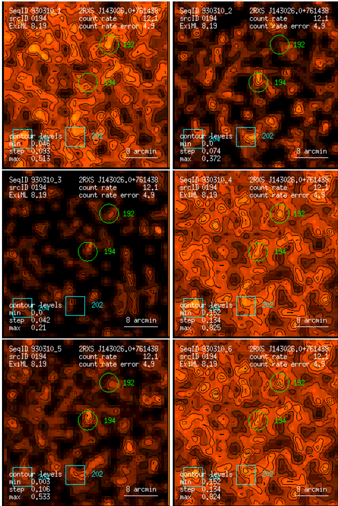
Figure 194: RASS 930310: detection 0194: band rate images, Gaussian filter: (1) PSPC channels 11 – 41, (2) 52 – 90, (3) 91 – 201, (4) 11 – 235, (5) 52 – 201, (6) 11 – 201. Broad band rates in counts/ks. Band rate contour levels in counts/ks/arcmin 2 .
