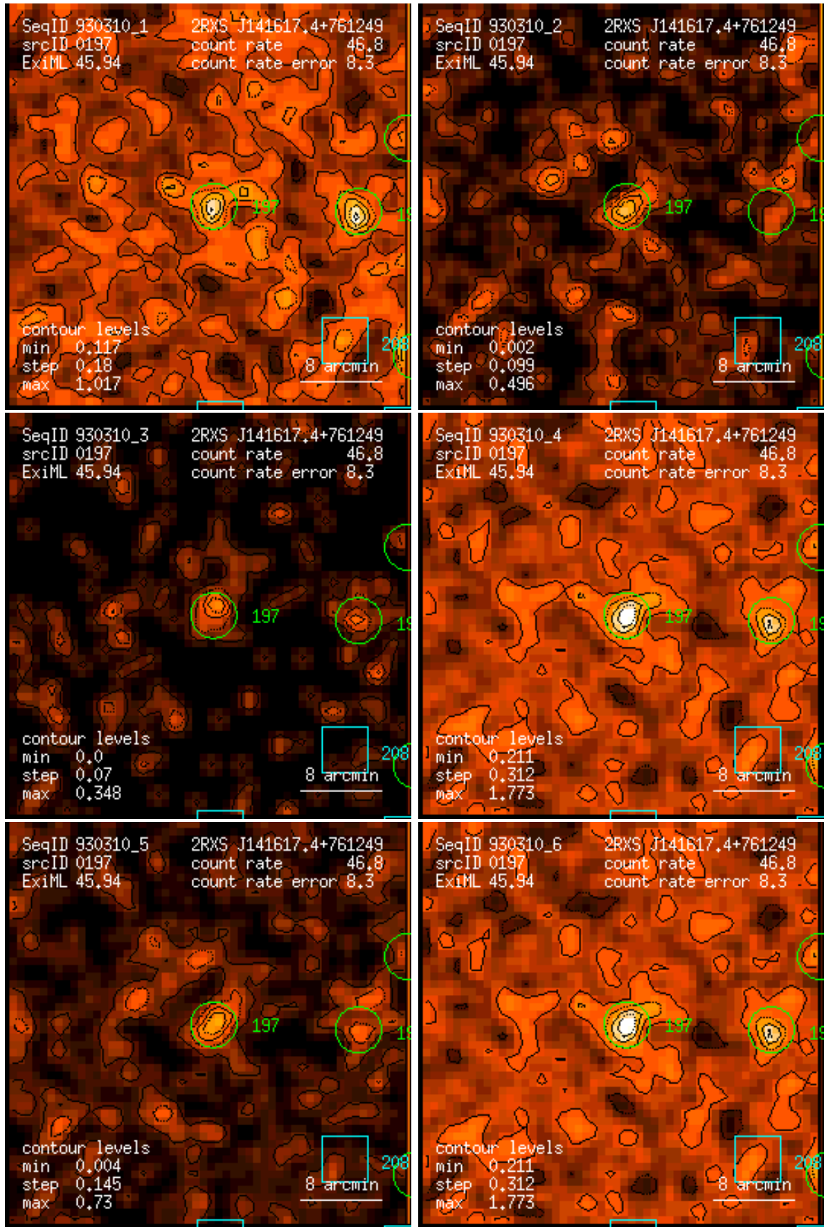
Figure 197: RASS 930310: detection 0197: band rate images, Gaussian filter: (1) PSPC channels 11 – 41, (2) 52 – 90, (3) 91 – 201, (4) 11 – 235, (5) 52 – 201, (6) 11 – 201. Broad band rates in counts/ks. Band rate contour levels in counts/ks/arcmin 2 .
