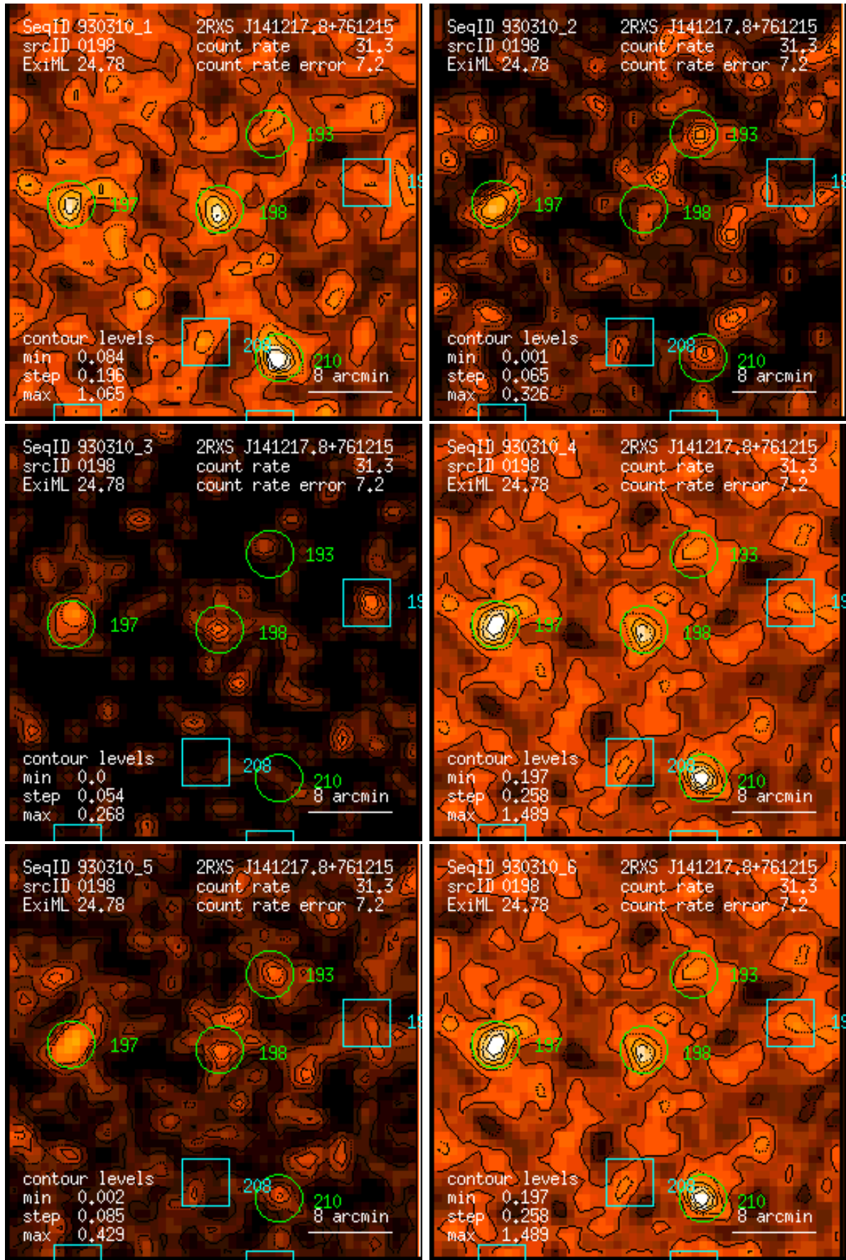
Figure 198: RASS 930310: detection 0198: band rate images, Gaussian filter: (1) PSPC channels 11 – 41, (2) 52 – 90, (3) 91 – 201, (4) 11 – 235, (5) 52 – 201, (6) 11 – 201. Broad band rates in counts/ks. Band rate contour levels in counts/ks/arcmin 2 .
