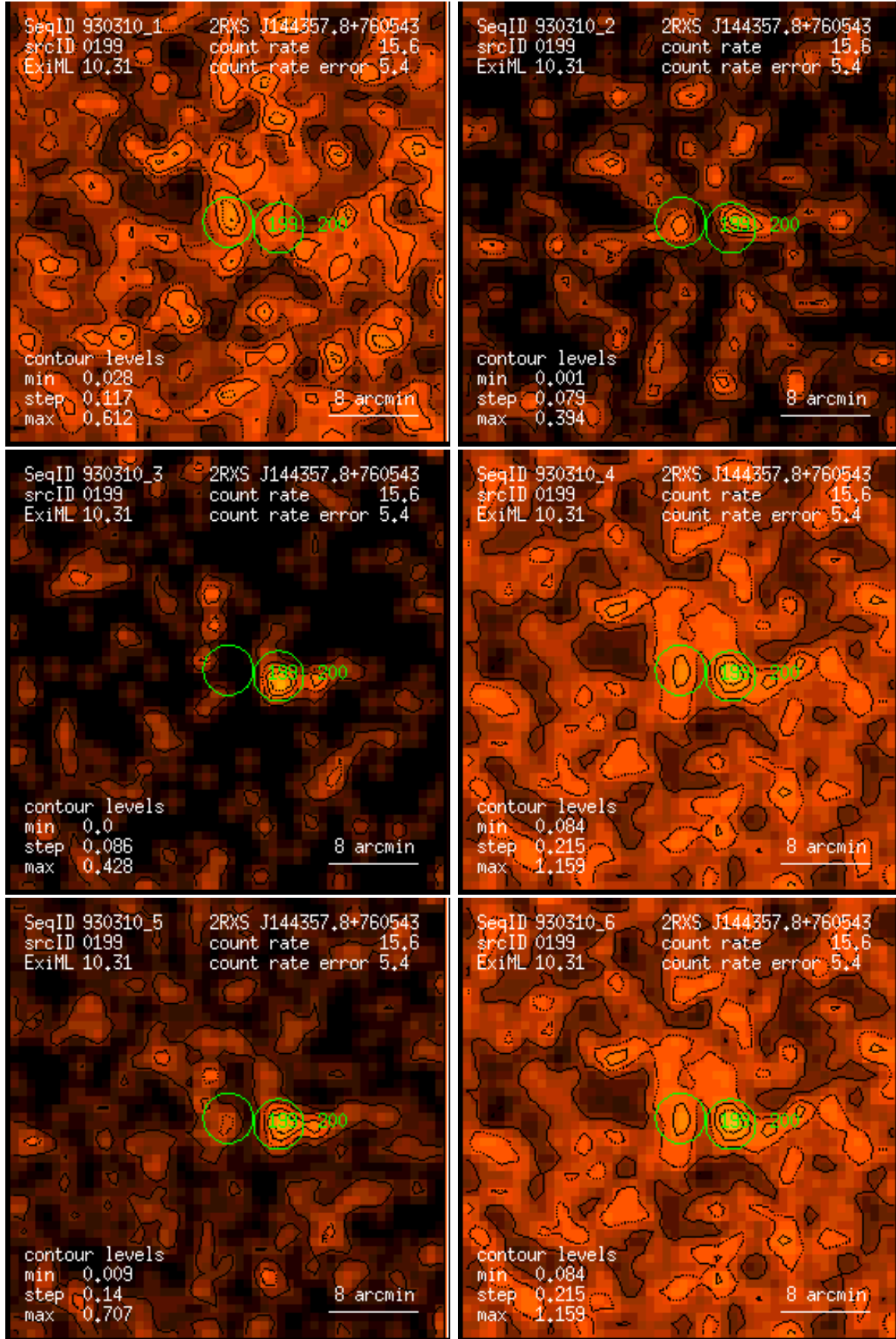
Figure 199: RASS 930310: detection 0199: band rate images, Gaussian filter: (1) PSPC channels 11 – 41, (2) 52 – 90, (3) 91 – 201, (4) 11 – 235, (5) 52 – 201, (6) 11 – 201. Broad band rates in counts/ks. Band rate contour levels in counts/ks/arcmin 2 .
