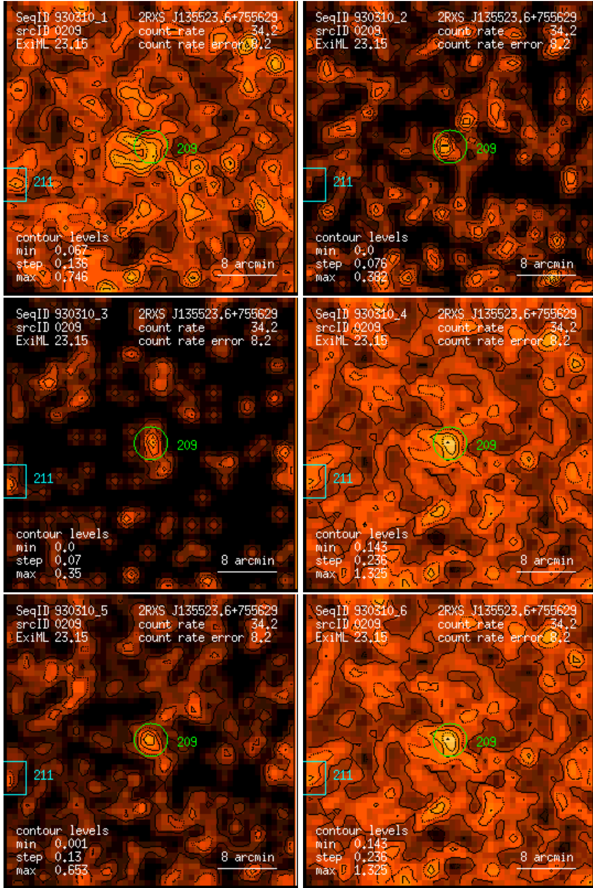
Figure 209: RASS 930310: detection 0209: band rate images, Gaussian filter: (1) PSPC channels 11 – 41, (2) 52 – 90, (3) 91 – 201, (4) 11 – 235, (5) 52 – 201, (6) 11 – 201. Broad band rates in counts/ks. Band rate contour levels in counts/ks/arcmin 2 .
