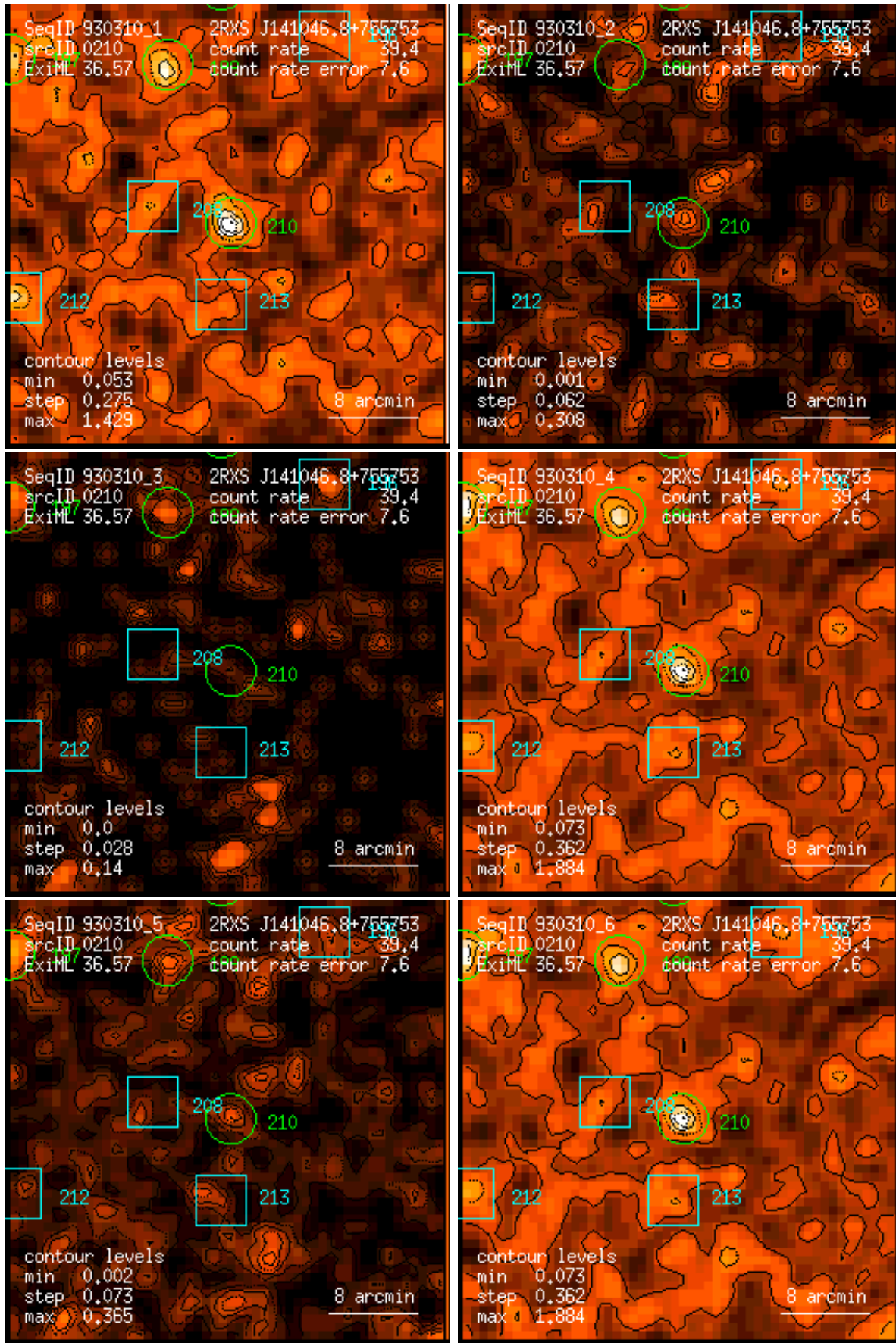
Figure 210: RASS 930310: detection 0210: band rate images, Gaussian filter: (1) PSPC channels 11 – 41, (2) 52 – 90, (3) 91 – 201, (4) 11 – 235, (5) 52 – 201, (6) 11 – 201. Broad band rates in counts/ks. Band rate contour levels in counts/ks/arcmin 2 .
