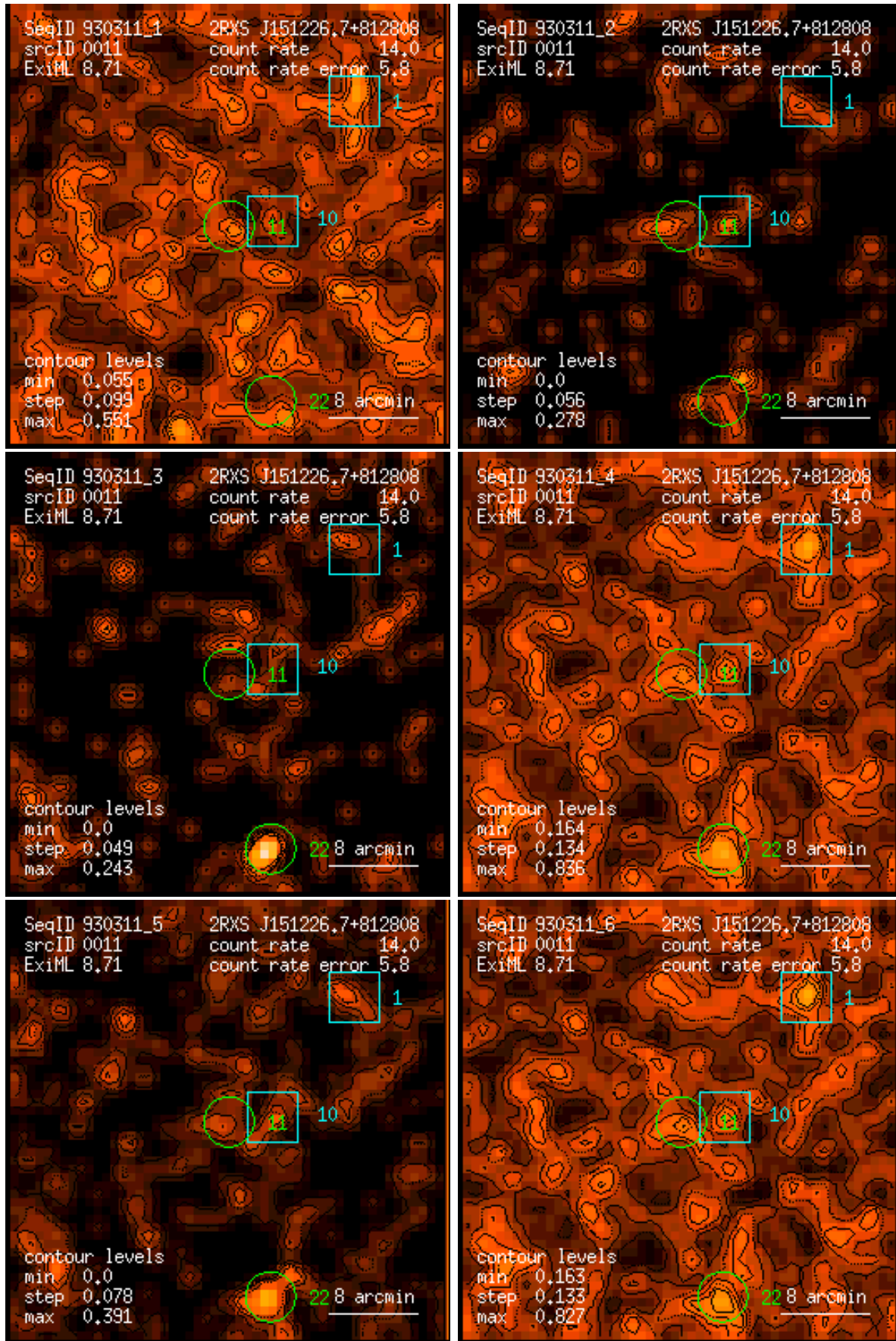
Figure 11: RASS 930311: detection 0011: band rate images, Gaussian filter: (1) PSPC channels 11 – 41, (2) 52 – 90, (3) 91 – 201, (4) 11 – 235, (5) 52 – 201, (6) 11 – 201. Broad band rates in counts/ks. Band rate contour levels in counts/ks/arcmin 2 .
