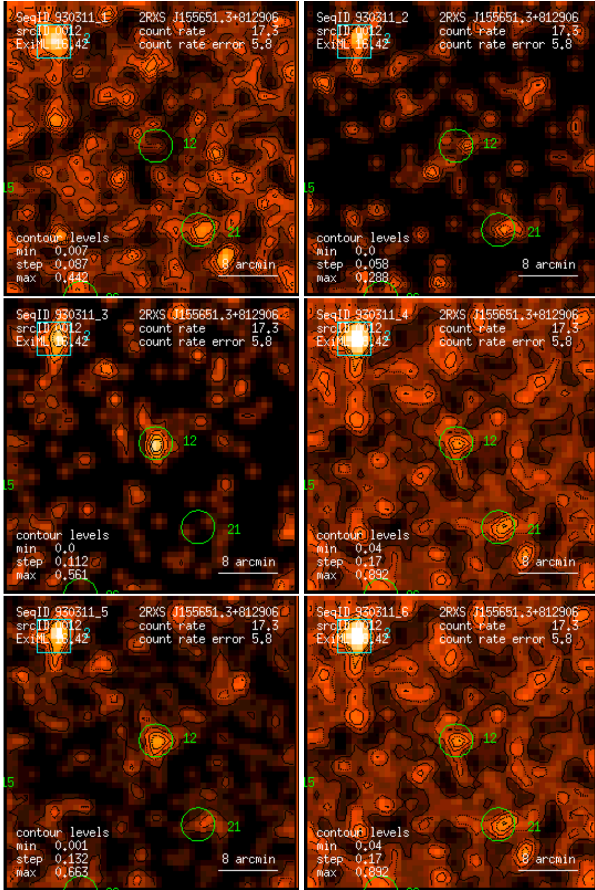
Figure 12: RASS 930311: detection 0012: band rate images, Gaussian filter: (1) PSPC channels 11 – 41, (2) 52 – 90, (3) 91 – 201, (4) 11 – 235, (5) 52 – 201, (6) 11 – 201. Broad band rates in counts/ks. Band rate contour levels in counts/ks/arcmin 2 .
