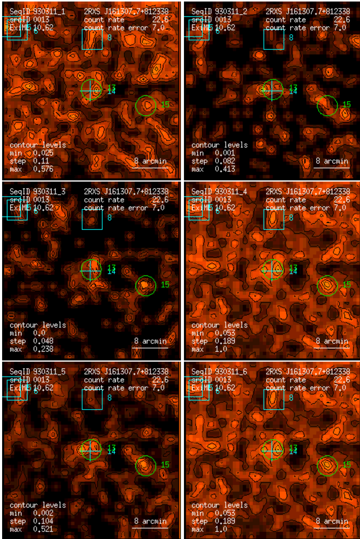
Figure 13: RASS 930311: detection 0013: band rate images, Gaussian filter: (1) PSPC channels 11 – 41, (2) 52 – 90, (3) 91 – 201, (4) 11 – 235, (5) 52 – 201, (6) 11 – 201. Broad band rates in counts/ks. Band rate contour levels in counts/ks/arcmin 2 .
