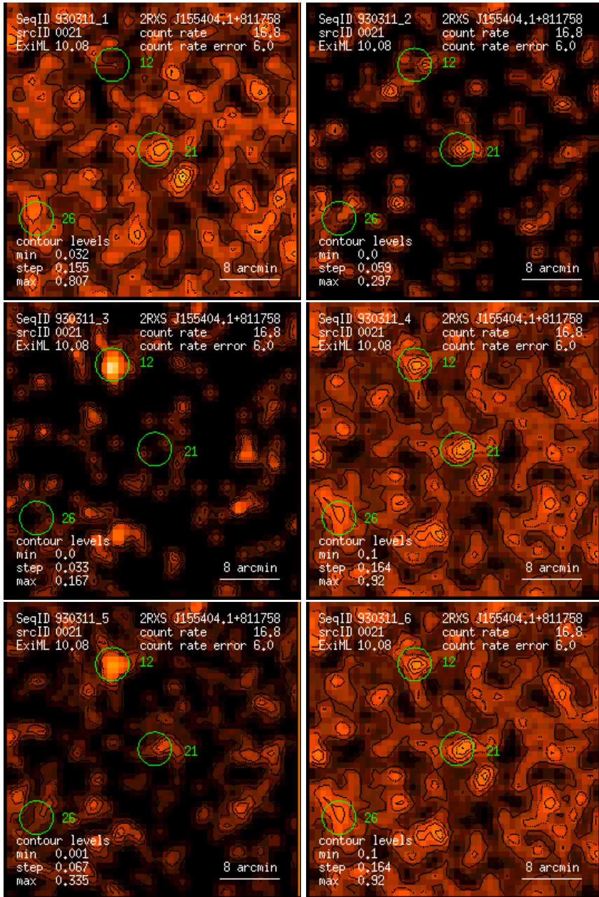
Figure 21: RASS 930311: detection 0021: band rate images, Gaussian filter: (1) PSPC channels 11 – 41, (2) 52 – 90, (3) 91 – 201, (4) 11 – 235, (5) 52 – 201, (6) 11 – 201. Broad band rates in counts/ks. Band rate contour levels in counts/ks/arcmin 2 .
