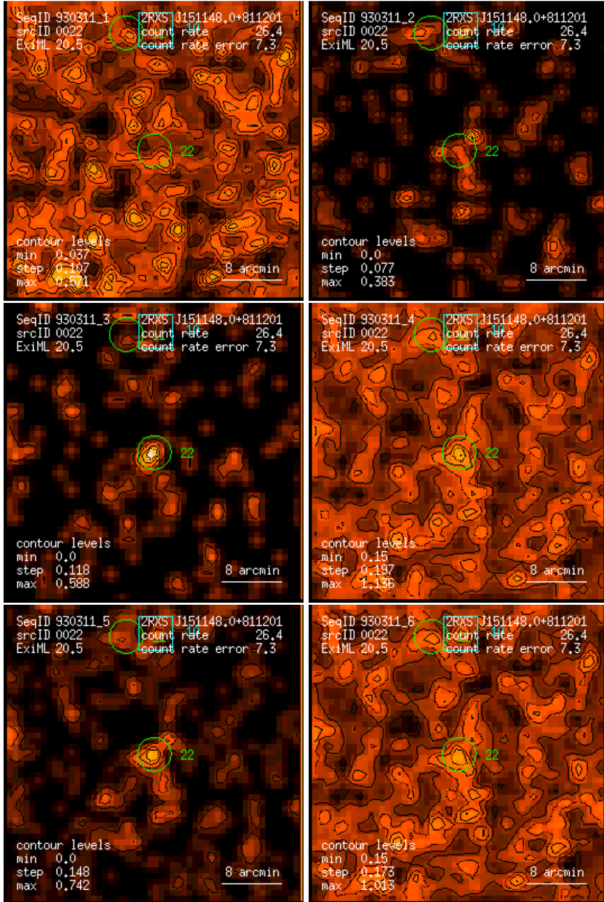
Figure 22: RASS 930311: detection 0022: band rate images, Gaussian filter: (1) PSPC channels 11 – 41, (2) 52 – 90, (3) 91 – 201, (4) 11 – 235, (5) 52 – 201, (6) 11 – 201. Broad band rates in counts/ks. Band rate contour levels in counts/ks/arcmin 2 .
