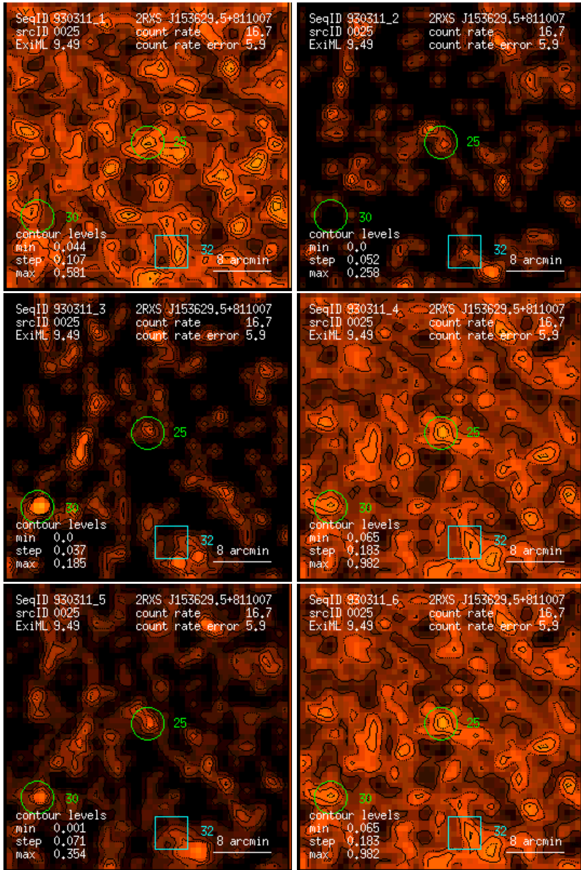
Figure 25: RASS 930311: detection 0025: band rate images, Gaussian filter: (1) PSPC channels 11 – 41, (2) 52 – 90, (3) 91 – 201, (4) 11 – 235, (5) 52 – 201, (6) 11 – 201. Broad band rates in counts/ks. Band rate contour levels in counts/ks/arcmin 2 .
